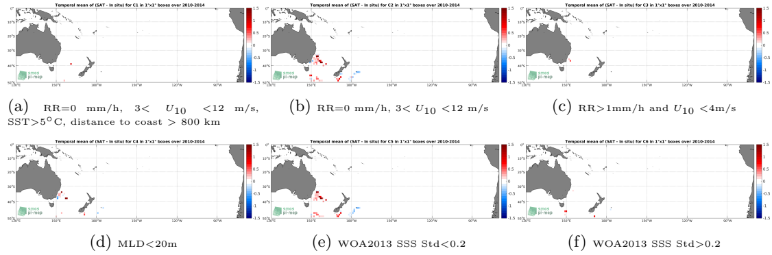
Figure 12: Temporal mean gridded over spatial boxes of size 1^\circ \times 1^\circ of \Delta SSS (SMOS SSS L3 v317 - Monthly - 25 km (CATDS-CPDC) - Marine mammals) for 6 different subdatasets corresponding to: RR=0 mm/h, 3 < U_{10} < 12 m/s, SST > 5^\circ C , distance to coast > 800 km (a), RR=0 mm/h, 3 < U_{10} < 12 m/s (b), RR > 1 mm/h and U_{10} < 4 m/s (c), MLD < 20 m (d), WOA2013 SSS Std < 0.2 (e), WOA2013 SSS Std > 0.2 (f).
