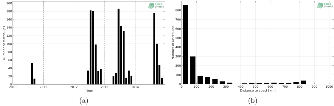
Figure 1: Number of match-ups between Marine mammals and SMOS SSS L3 v317 - Monthly - 25 km (CATDS-CPDC) SSS as a function of time (a) and as function of the distance to coast (b) over the South Pacific Ocean Pi-MEP region and for the full satellite product period.
