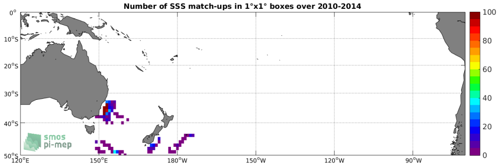
Figure 4: Number of SSS match-ups between Marine mammals SSS and the SMOS SSS L3 v317 - Monthly - 25 km (CATDS-CPDC) SSS product for the South Pacific Ocean Pi-MEP region over 1^\circ \times 1^\circ boxes and for the full satellite product period.
