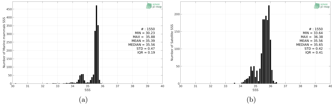
Figure 2: Histograms of SSS from Marine mammals (a) and SMOS SSS L3 v317 - Monthly - 25 km (CATDS-CPDC) (b) considering all match-up pairs per bins of 0.1 over the South Pacific Ocean Pi-MEP region and for the full satellite product period.
