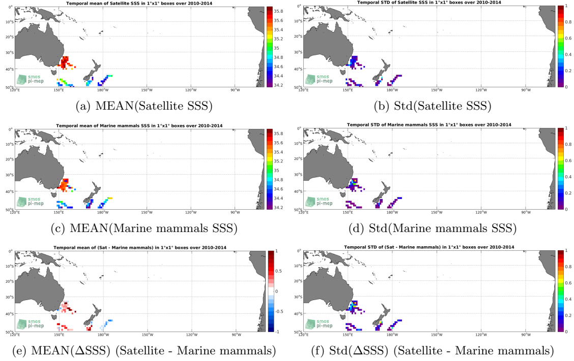
Figure 6: Temporal mean (left) and Std (right) of SSS from SMOS SSS L3 v317 - Monthly - 25 km (CATDS-CPDC) (top), Marine mammals (middle), and of \Delta SSS (Satellite - Marine mammals). Only match-up pairs are used to generate these maps.
