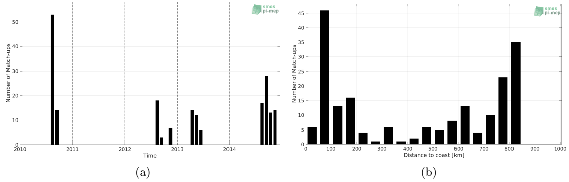
Figure 1: Number of match-ups between Sea mammals and SMOS SSS L3 v317 - Monthly - 25 km (CATDS-CPDC) SSS as a function of time (a) and as function of the distance to coast (b) over the South Pacific Ocean Pi-MEP region and for the full satellite product period.
