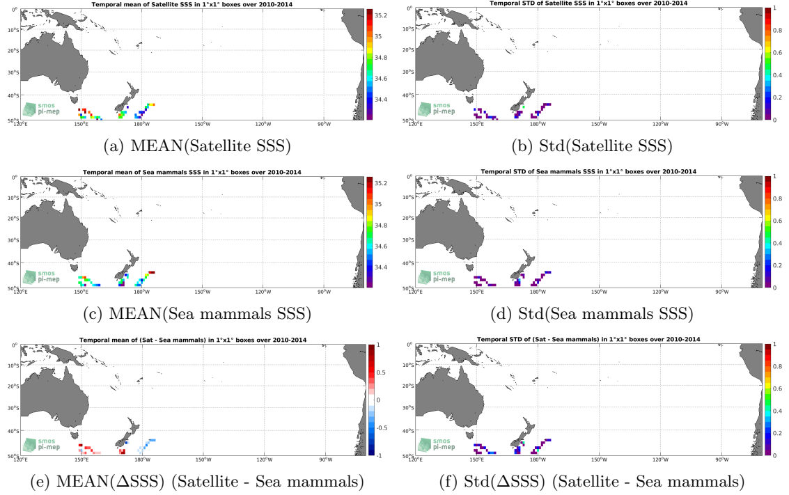
Figure 6: Temporal mean (left) and Std (right) of SSS from SMOS SSS L3 v317 - Monthly - 25 km (CATDS-CPDC) (top), Sea mammals (middle), and of \Delta SSS (Satellite - Sea mammals). Only match-up pairs are used to generate these maps.
