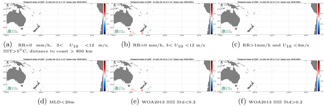
Figure 12: Temporal mean gridded over spatial boxes of size 1^{\circ}\times 1^{\circ} of \Delta\text{SSS} (SMOS SSS L3 v317 - Monthly - 25 km (CATDS-CPDC) - Sea mammals) for 6 different subdatasets corresponding to:RR=0 mm/h, 3 < U_{10} < 12 m/s, SST >5^{\circ}\text{C} , distance to coast > 800 km (a), RR=0 mm/h, 3 < U_{10} < 12 m/s (b), RR >1\text{mm/h} and U_{10} < 4\text{m/s} (c),MLD <20\text{m} (d),WOA2013 SSS Std <0.2 (e),WOA2013 SSS Std >0.2 (f).
