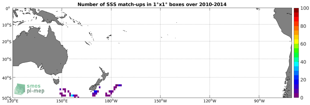
Figure 4: Number of SSS match-ups between Sea mammals SSS and the SMOS SSS L3 v317 - Monthly - 25 km (CATDS-CPDC) SSS product for the South Pacific Ocean Pi-MEP region over 1^\circ \times 1^\circ boxes and for the full satellite product period.
