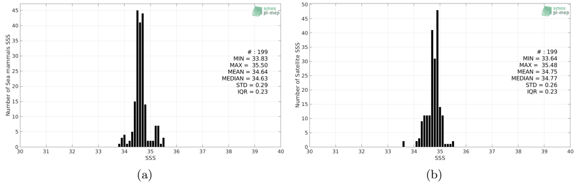
Figure 2: Histograms of SSS from Sea mammals (a) and SMOS SSS L3 v317 - Monthly - 25 km (CATDS-CPDC) (b) considering all match-up pairs per bins of 0.1 over the South Pacific Ocean Pi-MEP region and for the full satellite product period.
