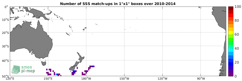
Figure 4: Number of SSS match-ups between Sea mammals SSS and the SMOS SSS L3 v317 - Monthly - 25 km (CATDS-CPDC) SSS product for the South Pacific Ocean Pi-MEP region over 1°x1° boxes and for the full satellite product period.
