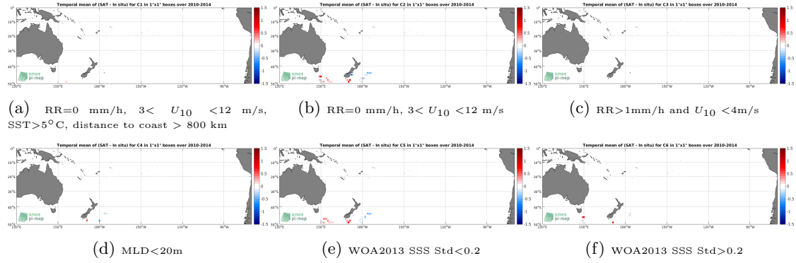
Figure 12: Temporal mean gridded over spatial boxes of size 1^\circ \times 1^\circ of \Delta SSS (SMOS-L3-CATDS-CPDC-V317-MONTHLY-25KM - Sea mammals) for 6 different subdatasets corresponding to: RR=0 mm/h, 3 < U_{10} < 12 m/s, SST >5^\circ\text{C} , distance to coast > 800 km (a), RR=0 mm/h, 3 < U_{10} < 12 m/s (b), RR>1\text{mm/h} and U_{10} < 4\text{m/s} (c), MLD<20\text{m} (d), WOA2013 SSS Std <0.2 (e), WOA2013 SSS Std >0.2 (f).
