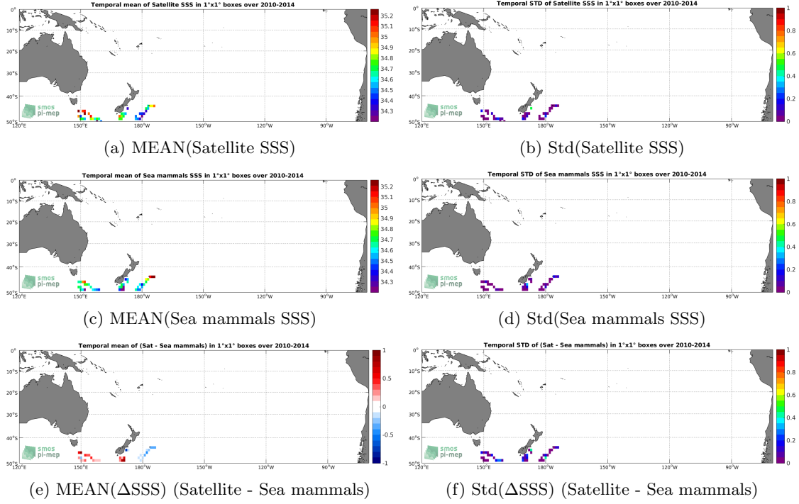
Figure 6: Temporal mean (left) and Std (right) of SSS from SMOS-L3-CATDS-CPDC-V317-MONTHLY-25KM (top), Sea mammals (middle), and of \Delta SSS (Satellite - Sea mammals). Only match-up pairs are used to generate these maps.
