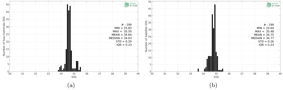
Figure 2: Histograms of SSS from Sea mammals (a) and SMOS-L3-CATDS-CPDC-V317-MONTHLY-25KM (b) considering all match-up pairs per bins of 0.1 over the South Pacific Ocean Pi-MEP region and for the full satellite product period.
