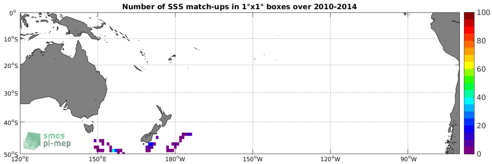
Figure 4: Number of SSS match-ups between Sea mammals SSS and the SMOS-L3-CATDS-CPDC-V317-MONTHLY-25KM SSS product for the South Pacific Ocean Pi-MEP region over 1^\circ \times 1^\circ boxes and for the full satellite product period.
