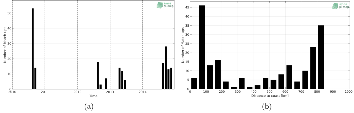
Figure 1: Number of match-ups between Sea mammals and SMOS-L3-CATDS-CPDC-V317-MONTHLY-25KM SSS as a function of time (a) and as function of the distance to coast (b) over the South Pacific Ocean Pi-MEP region and for the full satellite product period.
