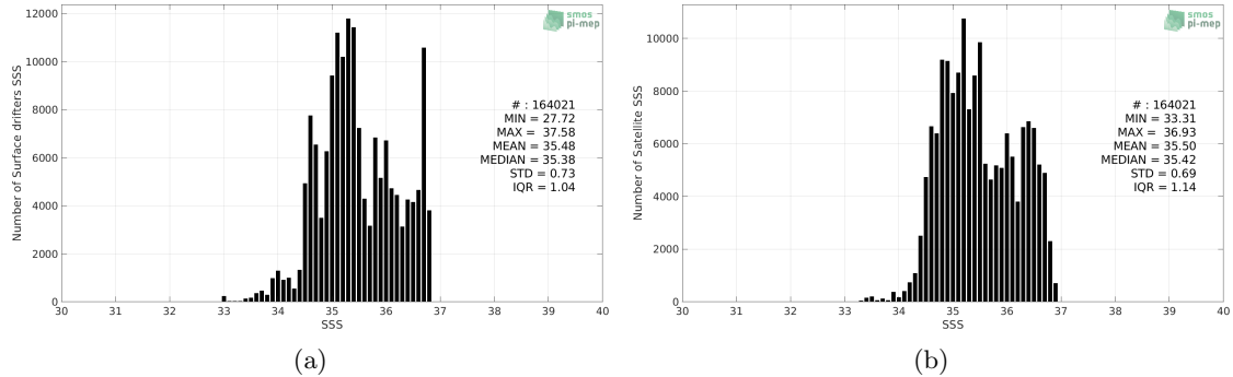
Figure 2: Histograms of SSS from Surface drifters (a) and SMOS SSS L3 v317 - Monthly - 25 km (CATDS-CPDC) (b) considering all match-up pairs per bins of 0.1 over the South Pacific Ocean Pi-MEP region and for the full satellite product period.
