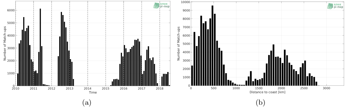
Figure 1: Number of match-ups between Surface drifters and SMOS SSS L3 v317 - Monthly - 25 km (CATDS-CPDC) SSS as a function of time (a) and as function of the distance to coast (b) over the South Pacific Ocean Pi-MEP region and for the full satellite product period.
