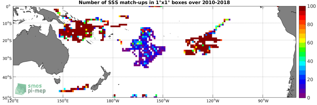
Figure 3: Number of SSS match-ups between Surface drifters SSS and the SMOS SSS L3 v317 - Monthly - 25 km (CATDS-CPDC) SSS product for the South Pacific Ocean Pi-MEP region over 1^\circ \times 1^\circ boxes and for the full satellite product period.
