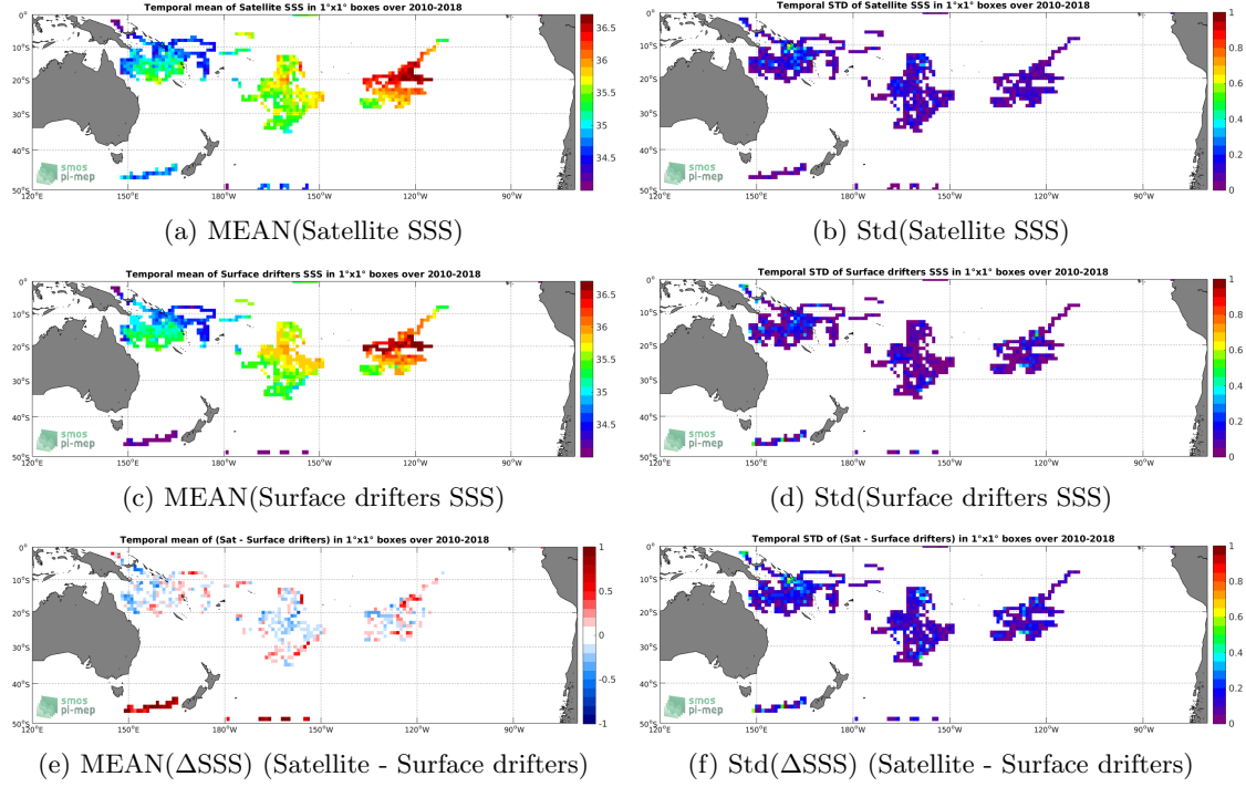
Figure 5: Temporal mean (left) and Std (right) of SSS from SMOS SSS L3 v317 - Monthly - 25 km (CATDS-CPDC) (top), Surface drifters (middle), and of \Delta SSS (Satellite - Surface drifters). Only match-up pairs are used to generate these maps.
