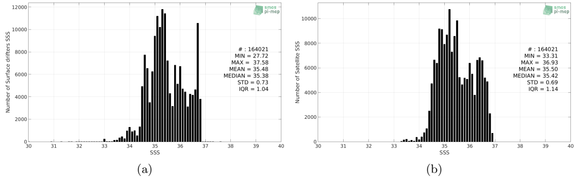
Figure 2: Histograms of SSS from Surface drifters (a) and SMOS SSS L3 v317 - Monthly - 25 km (CATDS-CPDC) (b) considering all match-up pairs per bins of 0.1 over the South Pacific Ocean Pi-MEP region and for the full satellite product period.
