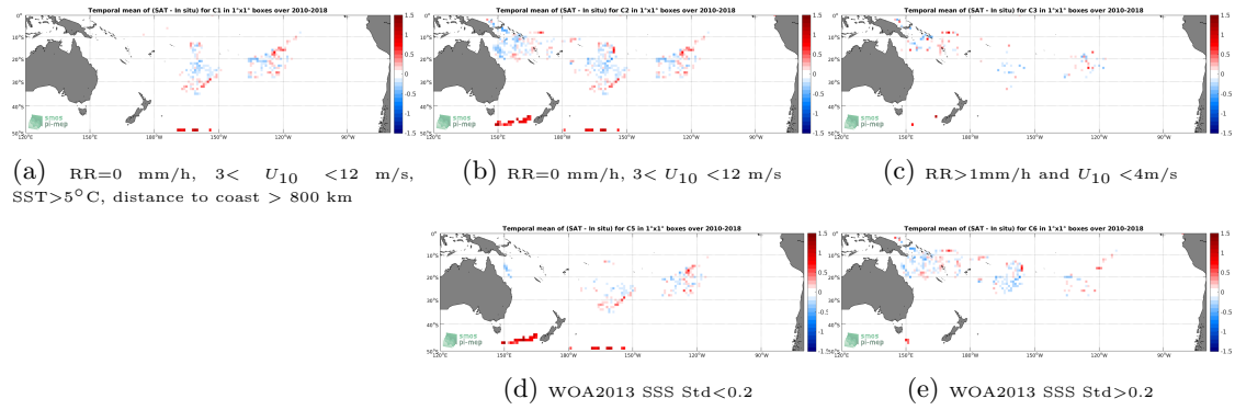
Figure 11: Temporal mean gridded over spatial boxes of size 1^\circ \times 1^\circ of \Delta SSS (SMOS SSS L3 v317 - Monthly - 25 km (CATDS-CPDC) - Surface drifters) for 5 different subdatasets corresponding to: RR=0 mm/h, 3 < U_{10} < 12 m/s, SST > 5^\circ\text{C} , distance to coast > 800 km (a), RR=0 mm/h, 3 < U_{10} < 12 m/s (b), RR > 1 mm/h and U_{10} < 4 m/s (c), WOA2013 SSS Std < 0.2 (d), WOA2013 SSS Std > 0.2 (e).
