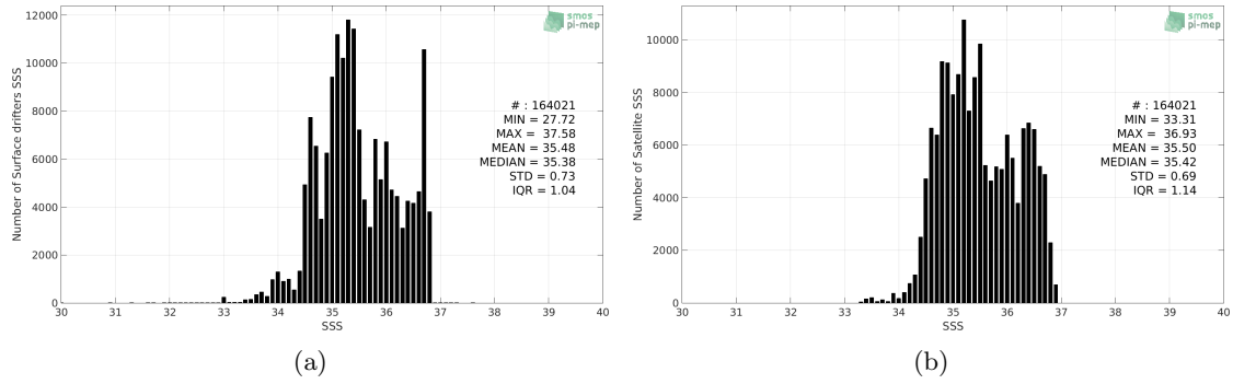
Figure 2: Histograms of SSS from Surface drifters (a) and SMOS L3 v317 - Monthly - 25 km (CATDS-CPDC) (b) considering all match-up pairs per bins of 0.1 over the South Pacific Ocean Pi-MEP region and for the full satellite product period.
