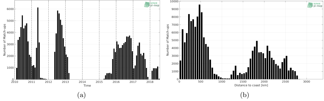
Figure 1: Number of match-ups between Surface drifters and SMOS L3 v317 - Monthly - 25 km (CATDS-CPDC) SSS as a function of time (a) and as function of the distance to coast (b) over the South Pacific Ocean Pi-MEP region and for the full satellite product period.
