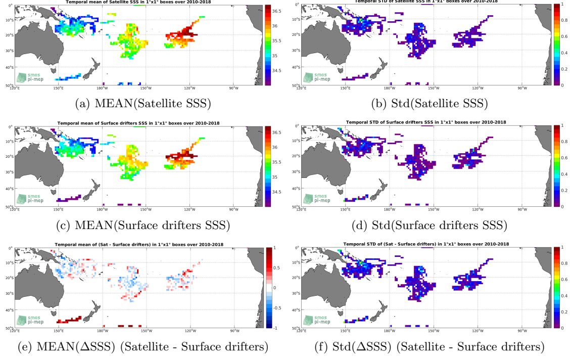
Figure 5: Temporal mean (left) and Std (right) of SSS from SMOS L3 v317 - Monthly - 25 km (CATDS-CPDC) (top), Surface drifters (middle), and of \Delta SSS (Satellite - Surface drifters). Only match-up pairs are used to generate these maps.
