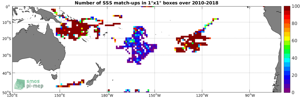
Figure 3: Number of SSS match-ups between Surface drifters SSS and the SMOS L3 v317 - Monthly - 25 km (CATDS-CPDC) SSS product for the South Pacific Ocean Pi-MEP region over 1°x1° boxes and for the full satellite product period.
