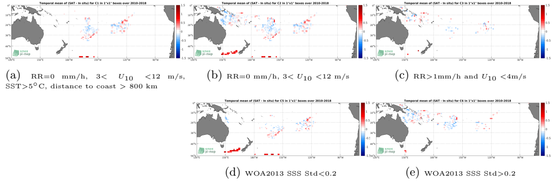
Figure 11: Temporal mean gridded over spatial boxes of size 1^\circ \times 1^\circ of \Delta SSS (SMOS L3 v317 - Monthly - 25 km (CATDS-CPDC) - Surface drifters) for 5 different subdatasets corresponding to: RR=0 mm/h, 3 < U_{10} < 12 m/s, SST > 5^\circ C , distance to coast > 800 km (a), RR=0 mm/h, 3 < U_{10} < 12 m/s (b), RR > 1 mm/h and U_{10} < 4 m/s (c), WOA2013 SSS Std < 0.2 (d), WOA2013 SSS Std > 0.2 (e).
