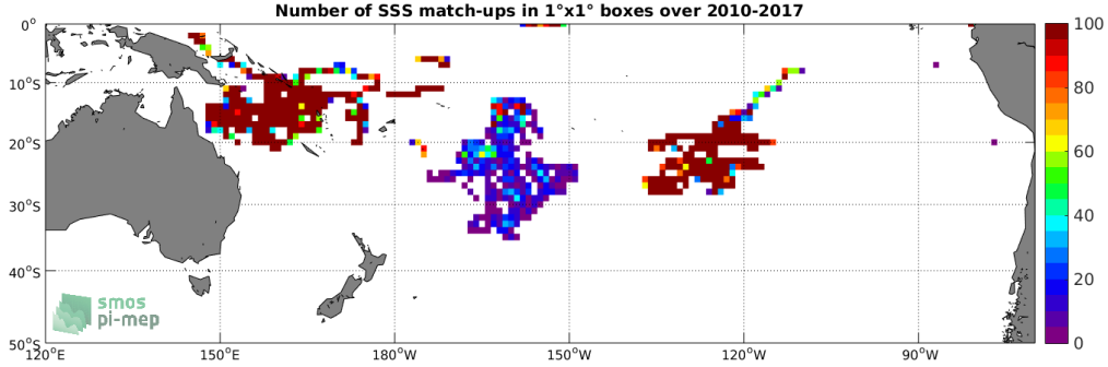
Figure 3: Number of SSS match-ups between Surface drifters SSS and the SMOS-L3-CATDS-CPDC-V317-MONTHLY-25KM SSS product for the South Pacific Ocean Pi-MEP region over 1°x1° boxes and for the full satellite product period.
