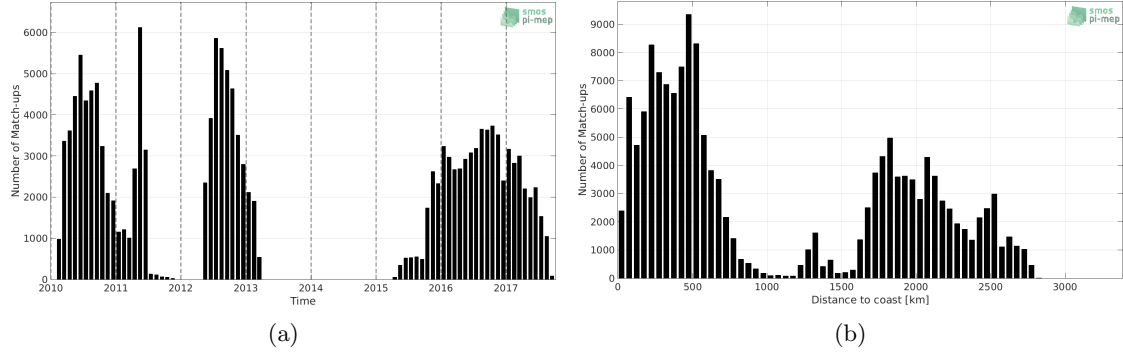
Figure 1: Number of match-ups between Surface drifters and SMOS-L3-CATDS-CPDC-V317-MONTHLY-25KM SSS as a function of time (a) and as function of the distance to coast (b) over the South Pacific Ocean Pi-MEP region and for the full satellite product period.
