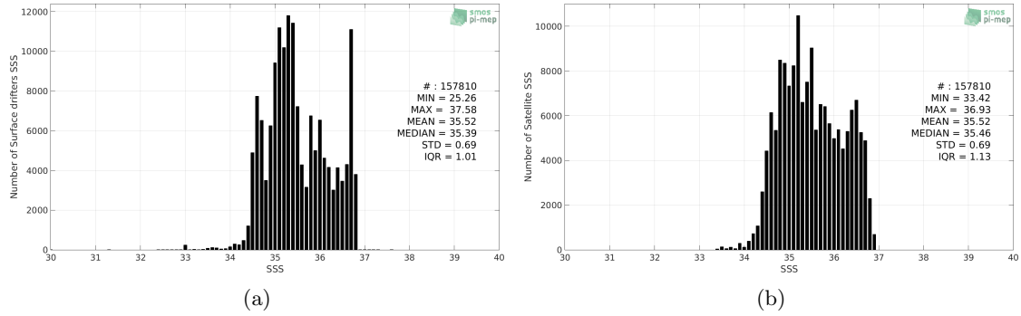
Figure 2: Histograms of SSS from Surface drifters (a) and SMOS-L3-CATDS-CPDC-V317-MONTHLY-25KM (b) considering all match-up pairs per bins of 0.1 over the South Pacific Ocean Pi-MEP region and for the full satellite product period.
