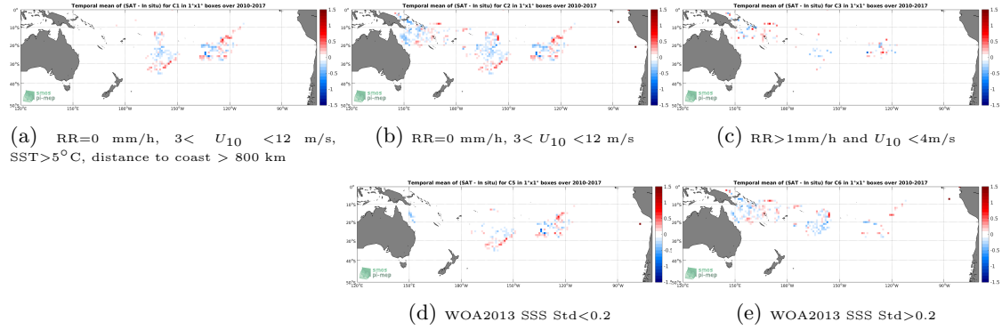
Figure 11: Temporal mean gridded over spatial boxes of size 1^\circ \times 1^\circ of \Delta SSS (SMOS-L3-CATDS-CPDC-V317-MONTHLY-25KM - Surface drifters) for 5 different subdatasets corresponding to: RR=0 mm/h, 3 < U_{10} < 12 m/s, SST > 5^\circ C , distance to coast > 800 km (a), RR=0 mm/h, 3 < U_{10} < 12 m/s (b), RR > 1 mm/h and U_{10} < 4 m/s (c), WOA2013 SSS Std < 0.2 (d), WOA2013 SSS Std > 0.2 (e).
