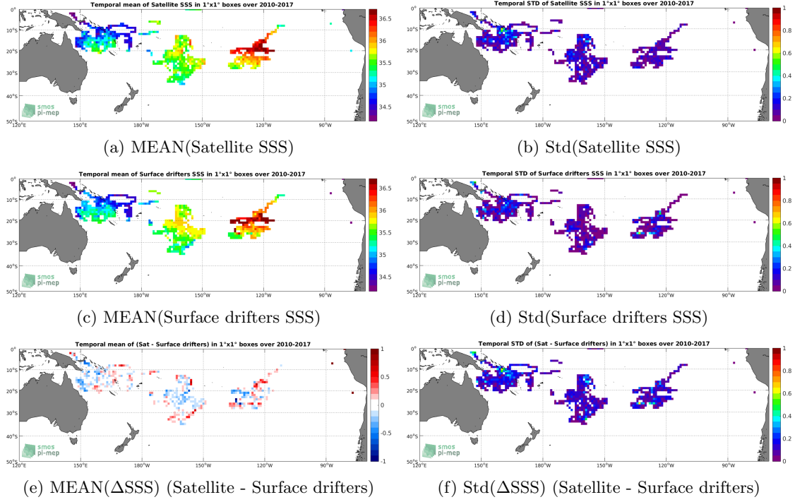
Figure 5: Temporal mean (left) and Std (right) of SSS from SMOS-L3-CATDS-CPDC-V317-MONTHLY-25KM (top), Surface drifters (middle), and of \Delta SSS (Satellite - Surface drifters). Only match-up pairs are used to generate these maps.
