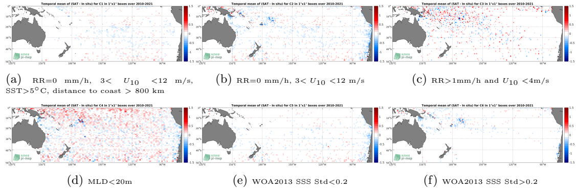
Figure 12: Temporal mean gridded over spatial boxes of size 1^\circ \times 1^\circ of \Delta SSS (SMOS SSS L3 v317 - Monthly - 25 km (CATDS-CPDC) - Argo) for 6 different subdatasets corresponding to: RR=0 mm/h, 3 < U_{10} < 12 m/s, SST > 5^\circ C , distance to coast > 800 km (a), RR=0 mm/h, 3 < U_{10} < 12 m/s (b), RR > 1 mm/h and U_{10} < 4 m/s (c), MLD < 20 m (d), WOA2013 SSS Std < 0.2 (e), WOA2013 SSS Std > 0.2 (f).
