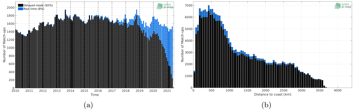
Figure 1: Number of match-ups between Argo and SMOS SSS L3 v317 - Monthly - 25 km (CATDS-CPDC) SSS as a function of time (a) and as function of the distance to coast (b) over the South Pacific Ocean Pi-MEP region and for the full satellite product period.
