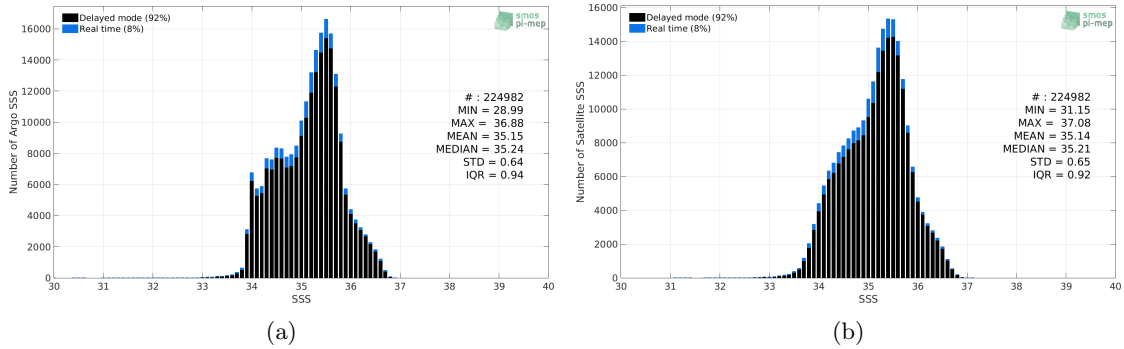
Figure 2: Histograms of SSS from Argo (a) and SMOS SSS L3 v317 - Monthly - 25 km (CATDS-CPDC) (b) considering all match-up pairs per bins of 0.1 over the South Pacific Ocean Pi-MEP region and for the full satellite product period.
