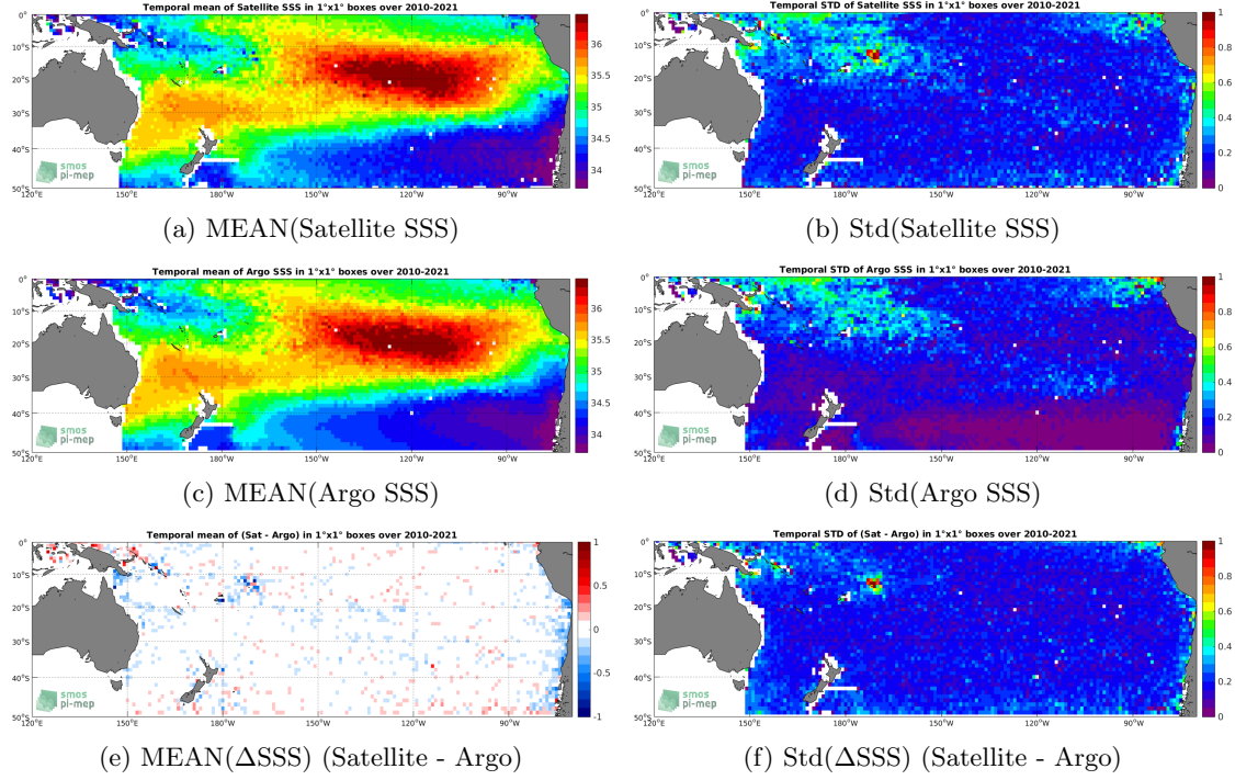
Figure 6: Temporal mean (left) and Std (right) of SSS from SMOS SSS L3 v317 - Monthly - 25 km (CATDS-CPDC) (top), Argo (middle), and of \Delta SSS (Satellite - Argo). Only match-up pairs are used to generate these maps.
