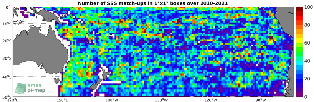
Figure 4: Number of SSS match-ups between Argo SSS and the SMOS SSS L3 v317 - Monthly - 25 km (CATDS-CPDC) SSS product for the South Pacific Ocean Pi-MEP region over 1^\circ \times 1^\circ boxes and for the full satellite product period.
