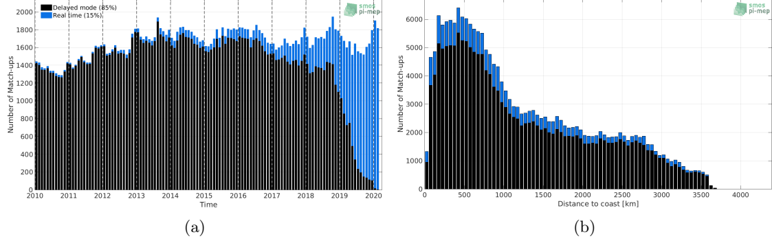
Figure 1: Number of match-ups between Argo and SMOS L3 v317 - Monthly - 25 km (CATDS-CPDC) SSS as a function of time (a) and as function of the distance to coast (b) over the South Pacific Ocean Pi-MEP region and for the full satellite product period.
