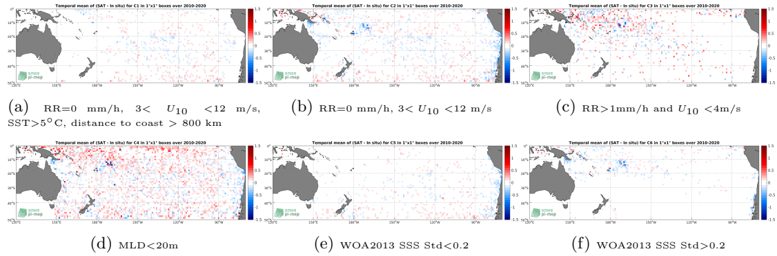
Figure 12: Temporal mean gridded over spatial boxes of size 1^\circ \times 1^\circ of \Delta SSS (SMOS L3 v317 - Monthly - 25 km (CATDS-CPDC) - Argo) for 6 different subdatasets corresponding to: RR=0 mm/h, 3 < U_{10} < 12 m/s, SST >5^\circ\text{C} , distance to coast > 800 km (a), RR=0 mm/h, 3 < U_{10} < 12 m/s (b), RR>1 mm/h and U_{10} < 4 m/s (c), MLD <20 m (d), WOA2013 SSS Std <0.2 (e), WOA2013 SSS Std >0.2 (f).
