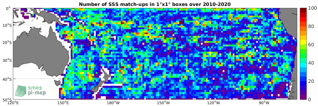
Figure 4: Number of SSS match-ups between Argo SSS and the SMOS L3 v317 - Monthly - 25 km (CATDS-CPDC) SSS product for the South Pacific Ocean Pi-MEP region over 1°x1° boxes and for the full satellite product period.
