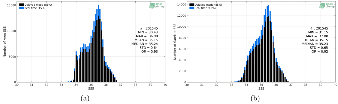
Figure 2: Histograms of SSS from Argo (a) and SMOS L3 v317 - Monthly - 25 km (CATDS-CPDC) (b) considering all match-up pairs per bins of 0.1 over the South Pacific Ocean Pi-MEP region and for the full satellite product period.
