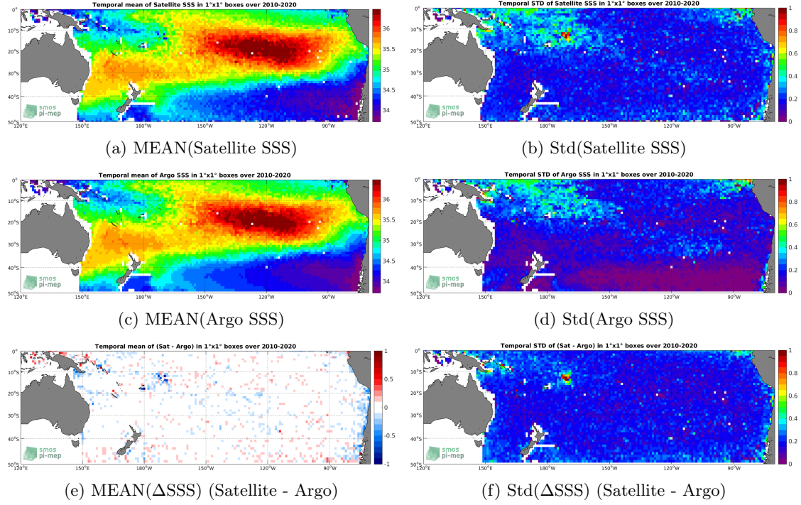
Figure 6: Temporal mean (left) and Std (right) of SSS from SMOS L3 v317 - Monthly - 25 km (CATDS-CPDC) (top), Argo (middle), and of \Delta SSS (Satellite - Argo). Only match-up pairs are used to generate these maps.
