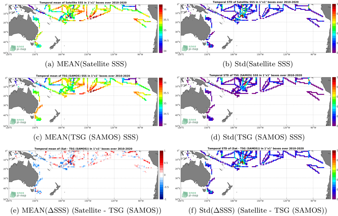
Figure 6: Temporal mean (left) and Std (right) of SSS from SMOS SSS L3 v317 - 10 Days - 25 km (CATDS-CPDC) (top), TSG (SAMOS) (middle), and of \Delta SSS (Satellite - TSG (SAMOS)). Only match-up pairs are used to generate these maps.
