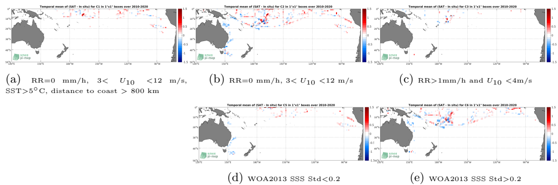
Figure 12: Temporal mean gridded over spatial boxes of size 1^\circ \times 1^\circ of \Delta SSS (SMOS SSS L3 v317 - 10 Days - 25 km (CATDS-CPDC) - TSG (SAMOS)) for 5 different subdatasets corresponding to:RR=0 mm/h, 3 < U_{10} < 12 m/s, SST >5^\circ C, distance to coast > 800 km (a), RR=0 mm/h, 3 < U_{10} < 12 m/s (b), RR >1 mm/h and U_{10} < 4 m/s (c), WOA2013 SSS Std <0.2 (d), WOA2013 SSS Std >0.2 (e).
