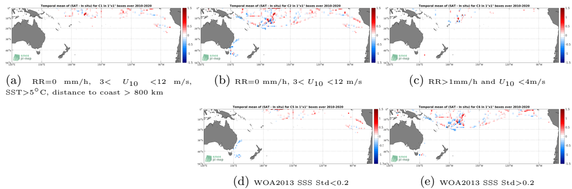
Figure 12: Temporal mean gridded over spatial boxes of size 1^\circ \times 1^\circ of \Delta SSS (SMOS L3 v317 - 10 Days - 25 km (CATDS-CPDC) - TSG-SAMOS) for 5 different subdatasets corresponding to:RR=0 mm/h, 3 < U_{10} < 12 m/s, SST >5^\circ\text{C} , distance to coast > 800 km (a), RR=0 mm/h, 3 < U_{10} < 12 m/s (b), RR >1 mm/h and U_{10} < 4 m/s (c), WOA2013 SSS Std <0.2 (d), WOA2013 SSS Std >0.2 (e).
