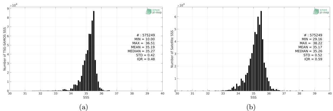
Figure 2: Histograms of SSS from TSG-SAMOS (a) and SMOS L3 v317 - 10 Days - 25 km (CATDS-CPDC) (b) considering all match-up pairs per bins of 0.1 over the South Pacific Ocean Pi-MEP region and for the full satellite product period.
