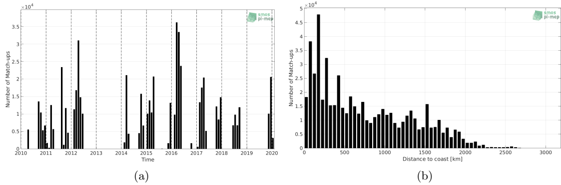
Figure 1: Number of match-ups between TSG-SAMOS and SMOS L3 v317 - 10 Days - 25 km (CATDS-CPDC) SSS as a function of time (a) and as function of the distance to coast (b) over the South Pacific Ocean Pi-MEP region and for the full satellite product period.
