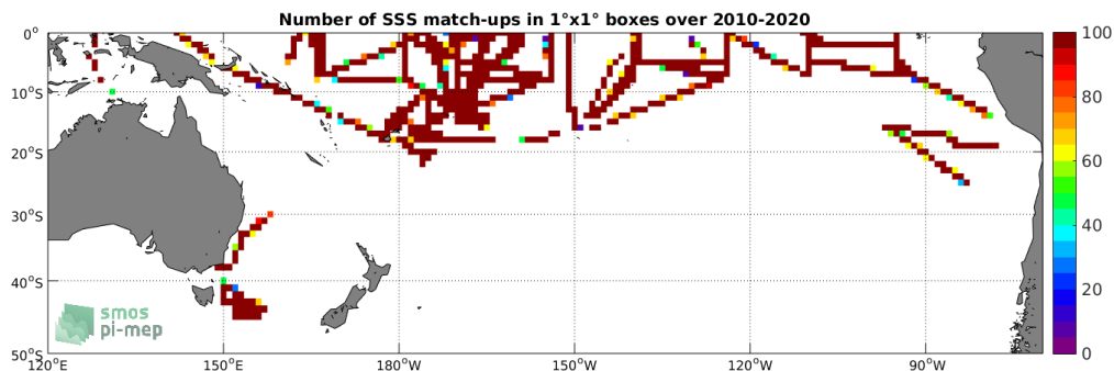
Figure 4: Number of SSS match-ups between TSG-SAMOS SSS and the SMOS L3 v317 - 10 Days - 25 km (CATDS-CPDC) SSS product for the South Pacific Ocean Pi-MEP region over 1^\circ \times 1^\circ boxes and for the full satellite product period.
