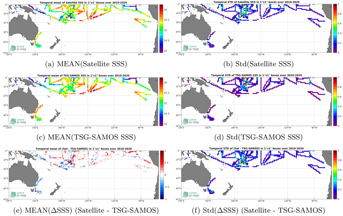
Figure 6: Temporal mean (left) and Std (right) of SSS from SMOS L3 v317 - 10 Days - 25 km (CATDS-CPDC) (top), TSG-SAMOS (middle), and of \Delta SSS (Satellite - TSG-SAMOS). Only match-up pairs are used to generate these maps.
