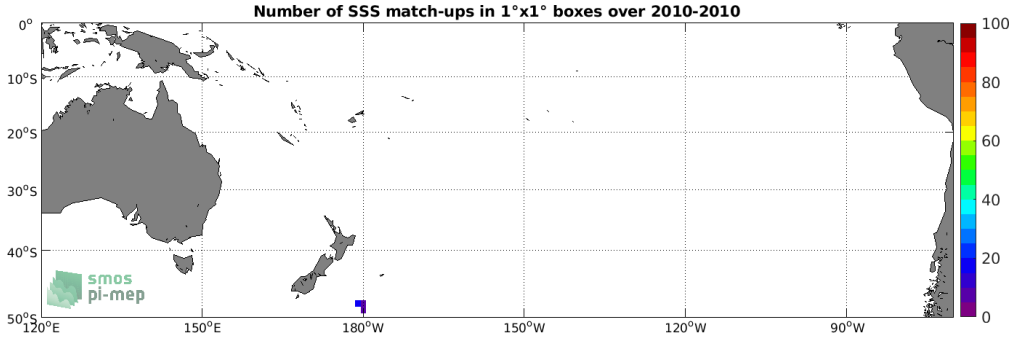
Figure 4: Number of SSS match-ups between TSG (Polarstern) SSS and the SMOS SSS L3 v317 - 10 Days - 25 km (CATDS-CPDC) SSS product for the South Pacific Ocean Pi-MEP region over 1^\circ \times 1^\circ boxes and for the full satellite product period.
