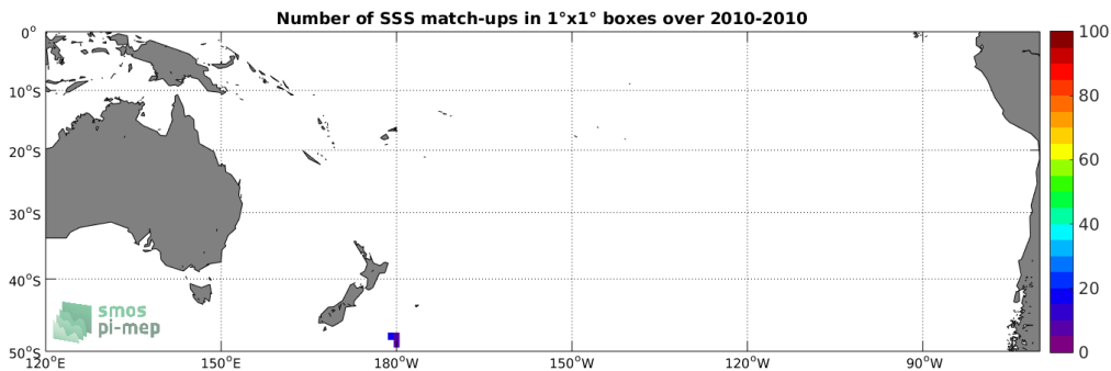
Figure 4: Number of SSS match-ups between TSG (Polarstern) SSS and the SMOS SSS L3 v317 - 10 Days - 25 km (CATDS-CPDC) SSS product for the South Pacific Ocean Pi-MEP region over 1°x1° boxes and for the full satellite product period.
