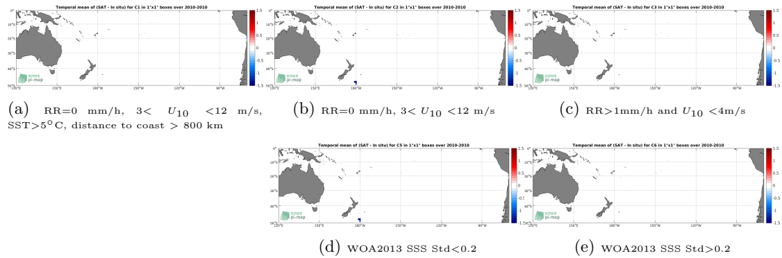
Figure 12: Temporal mean gridded over spatial boxes of size 1^{\circ}\times 1^{\circ} of \Delta\text{SSS} (SMOS SSS L3 v317 - 10 Days - 25 km (CATDS-CPDC) - TSG (Polarstern)) for 5 different subdatasets corresponding to:RR=0 mm/h, 3 < U_{10} < 12 m/s, SST >5^{\circ}\text{C} , distance to coast > 800 km (a), RR=0 mm/h, 3 < U_{10} < 12 m/s (b), RR >1 mm/h and U_{10} < 4 m/s (c), WOA2013 SSS Std <0.2 (d), WOA2013 SSS Std >0.2 (e).
