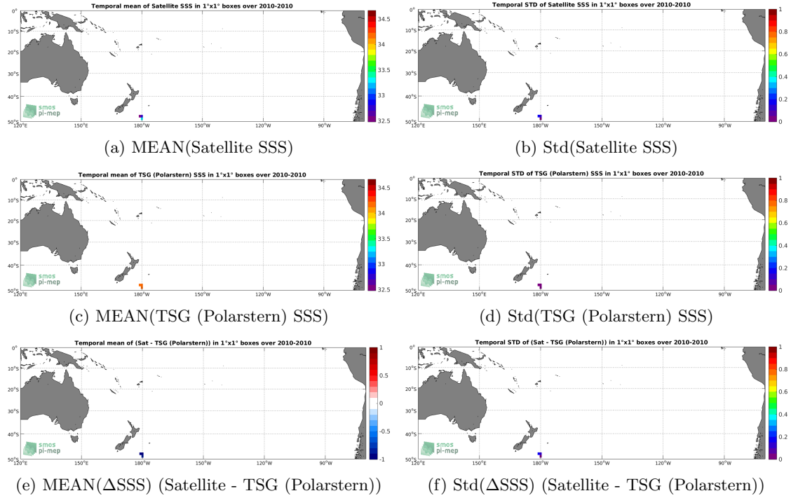
Figure 6: Temporal mean (left) and Std (right) of SSS from SMOS SSS L3 v317 - 10 Days - 25 km (CATDS-CPDC) (top), TSG (Polarstern) (middle), and of \Delta SSS (Satellite - TSG (Polarstern)). Only match-up pairs are used to generate these maps.
