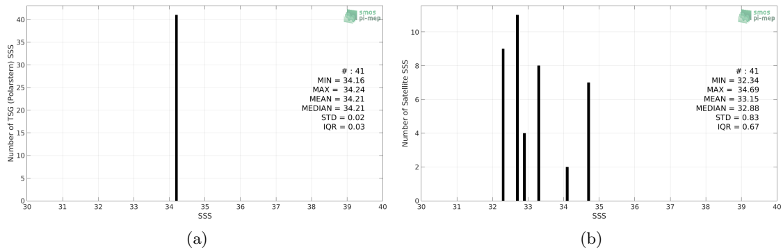
Figure 2: Histograms of SSS from TSG (Polarstern) (a) and SMOS SSS L3 v317 - 10 Days - 25 km (CATDS-CPDC) (b) considering all match-up pairs per bins of 0.1 over the South Pacific Ocean Pi-MEP region and for the full satellite product period.
