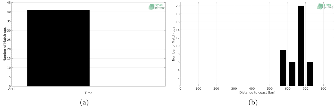
Figure 1: Number of match-ups between TSG (Polarstern) and SMOS SSS L3 v317 - 10 Days - 25 km (CATDS-CPDC) SSS as a function of time (a) and as function of the distance to coast (b) over the South Pacific Ocean Pi-MEP region and for the full satellite product period.
