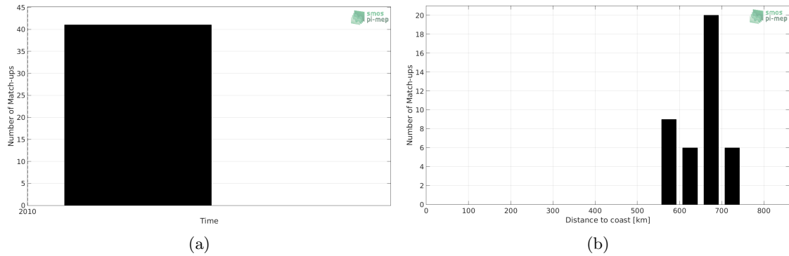
Figure 1: Number of match-ups between TSG-POLARSTERN and SMOS L3 v317 - 10 Days - 25 km (CATDS-CPDC) SSS as a function of time (a) and as function of the distance to coast (b) over the South Pacific Ocean Pi-MEP region and for the full satellite product period.
