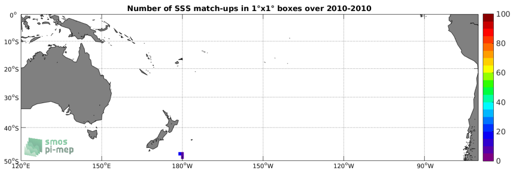
Figure 4: Number of SSS match-ups between TSG-POLARSTERN SSS and the SMOS L3 v317 - 10 Days - 25 km (CATDS-CPDC) SSS product for the South Pacific Ocean Pi-MEP region over 1^\circ \times 1^\circ boxes and for the full satellite product period.
