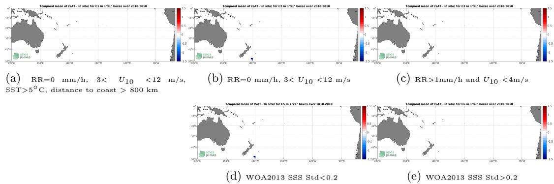
Figure 12: Temporal mean gridded over spatial boxes of size 1^{\circ}\times 1^{\circ} of \Delta\text{SSS} (SMOS L3 v317 - 10 Days - 25 km (CATDS-CPDC) - TSG-POLARSTERN) for 5 different subdatasets corresponding to:RR=0 mm/h, 3 < U_{10} < 12 m/s, SST >5^{\circ}\text{C} , distance to coast > 800 km (a), RR=0 mm/h, 3 < U_{10} < 12 m/s (b), RR >1 mm/h and U_{10} < 4 m/s (c), WOA2013 SSS Std <0.2 (d), WOA2013 SSS Std >0.2 (e).
