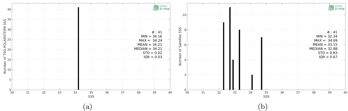
Figure 2: Histograms of SSS from TSG-POLARSTERN (a) and SMOS L3 v317 - 10 Days - 25 km (CATDS-CPDC) (b) considering all match-up pairs per bins of 0.1 over the South Pacific Ocean Pi-MEP region and for the full satellite product period.
