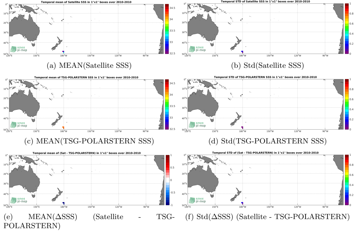
Figure 6: Temporal mean (left) and Std (right) of SSS from SMOS-L3-CATDS-CPDC-V317-10DAYS-25KM (top), TSG-POLARSTERN (middle), and of \Delta SSS (Satellite - TSG-POLARSTERN). Only match-up pairs are used to generate these maps.
