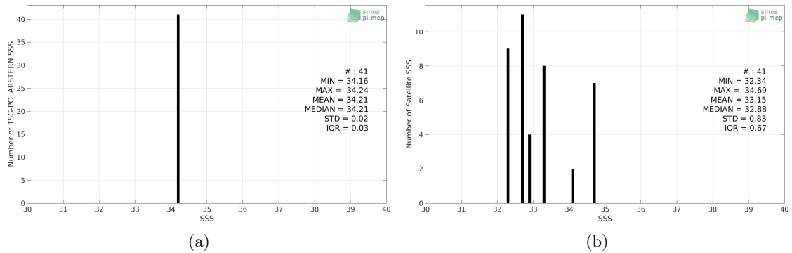
Figure 2: Histograms of SSS from TSG-POLARSTERN (a) and SMOS-L3-CATDS-CPDC-V317-10DAYS-25KM (b) considering all match-up pairs per bins of 0.1 over the South Pacific Ocean Pi-MEP region and for the full satellite product period.
