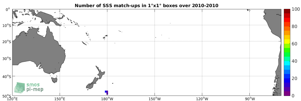
Figure 4: Number of SSS match-ups between TSG-POLARSTERN SSS and the SMOS-L3-CATDS-CPDC-V317-10DAYS-25KM SSS product for the South Pacific Ocean Pi-MEP region over 1^\circ \times 1^\circ boxes and for the full satellite product period.
