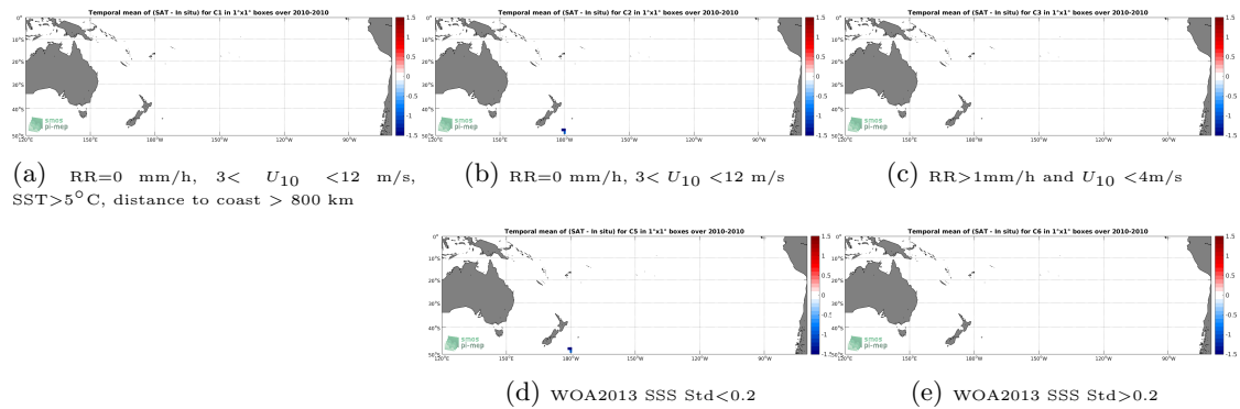
Figure 12: Temporal mean gridded over spatial boxes of size 1^\circ \times 1^\circ of \Delta SSS (SMOS-L3-CATDS-CPDC-V317-10DAYS-25KM - TSG-POLARSTERN) for 5 different subdatasets corresponding to:RR=0 mm/h, 3 < U_{10} < 12 m/s, SST >5^\circ\text{C} , distance to coast > 800 km (a), RR=0 mm/h, 3 < U_{10} < 12 m/s (b), RR >1 mm/h and U_{10} < 4 m/s (c), WOA2013 SSS Std <0.2 (d), WOA2013 SSS Std >0.2 (e).
