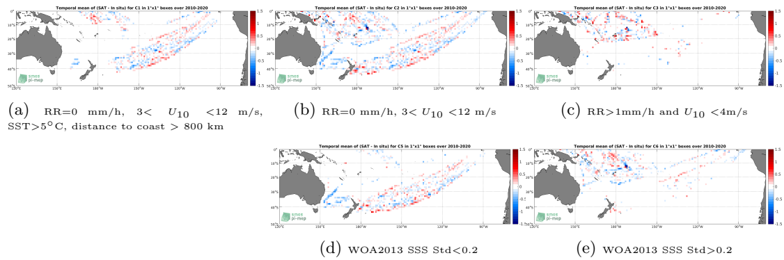
Figure 12: Temporal mean gridded over spatial boxes of size 1^\circ \times 1^\circ of \Delta\text{SSS} (SMOS SSS L3 v317 - 10 Days - 25 km (CATDS-CPDC) - TSG (LEGOS-DM)) for 5 different subdatasets corresponding to:RR=0 mm/h, 3 < U_{10} < 12 m/s, SST >5^\circ\text{C} , distance to coast > 800 km (a), RR=0 mm/h, 3 < U_{10} < 12 m/s (b), RR >1 mm/h and U_{10} < 4 m/s (c), WOA2013 SSS Std <0.2 (d), WOA2013 SSS Std >0.2 (e).
