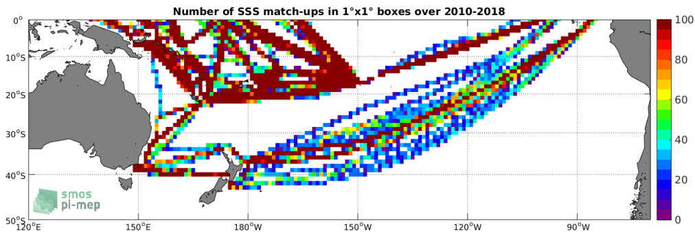
Figure 4: Number of SSS match-ups between TSG-LEGOS-DM SSS and the SMOS-L3-CATDS-CPDC-V317-10DAYS-25KM SSS product for the South Pacific Ocean Pi-MEP region over 1^\circ \times 1^\circ boxes and for the full satellite product period.
