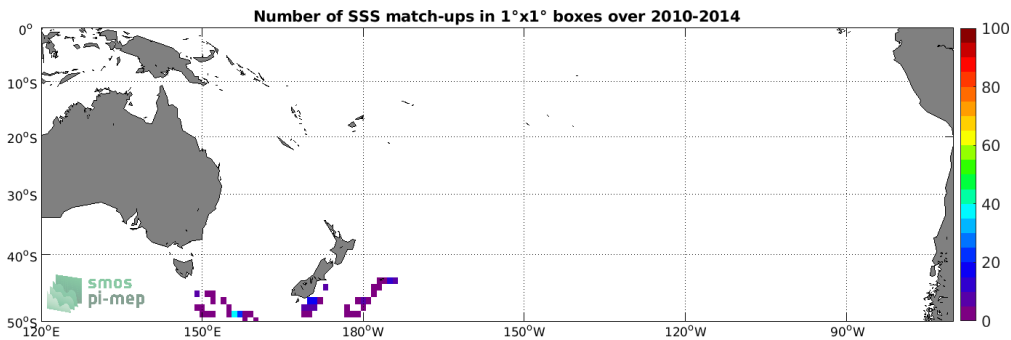
Figure 4: Number of SSS match-ups between Sea mammals SSS and the SMOS SSS L3 v317 - 10 Days - 25 km (CATDS-CPDC) SSS product for the South Pacific Ocean Pi-MEP region over 1^\circ \times 1^\circ boxes and for the full satellite product period.
