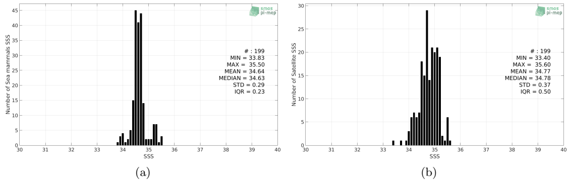
Figure 2: Histograms of SSS from Sea mammals (a) and SMOS SSS L3 v317 - 10 Days - 25 km (CATDS-CPDC) (b) considering all match-up pairs per bins of 0.1 over the South Pacific Ocean Pi-MEP region and for the full satellite product period.
