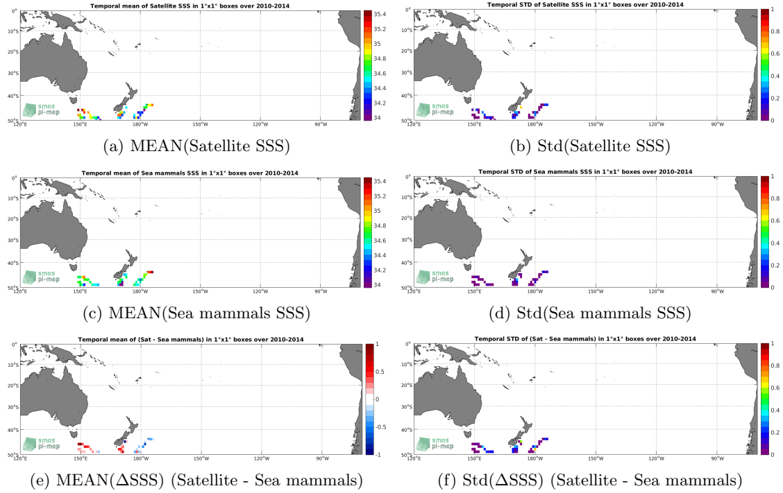
Figure 6: Temporal mean (left) and Std (right) of SSS from SMOS SSS L3 v317 - 10 Days - 25 km (CATDS-CPDC) (top), Sea mammals (middle), and of \Delta SSS (Satellite - Sea mammals). Only match-up pairs are used to generate these maps.
