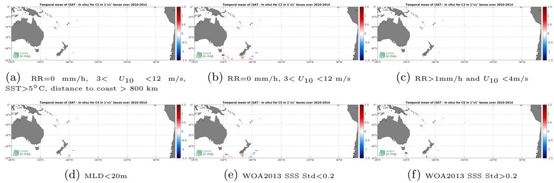
Figure 12: Temporal mean gridded over spatial boxes of size 1^{\circ}\times 1^{\circ} of \Delta\text{SSS} (SMOS SSS L3 v317 - 10 Days - 25 km (CATDS-CPDC) - Sea mammals) for 6 different subdatasets corresponding to:RR=0 mm/h, 3 < U_{10} < 12 m/s, SST >5^{\circ}\text{C} , distance to coast > 800 km (a), RR=0 mm/h, 3 < U_{10} < 12 m/s (b), RR >1\text{mm/h} and U_{10} < 4\text{m/s} (c),MLD <20\text{m} (d),WOA2013 SSS Std <0.2 (e),WOA2013 SSS Std >0.2 (f).
