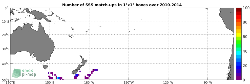
Figure 4: Number of SSS match-ups between Sea mammals SSS and the SMOS SSS L3 v317 - 10 Days - 25 km (CATDS-CPDC) SSS product for the South Pacific Ocean Pi-MEP region over 1°x1° boxes and for the full satellite product period.
