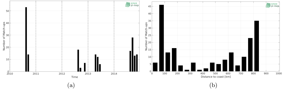
Figure 1: Number of match-ups between Sea mammals and SMOS SSS L3 v317 - 10 Days - 25 km (CATDS-CPDC) SSS as a function of time (a) and as function of the distance to coast (b) over the South Pacific Ocean Pi-MEP region and for the full satellite product period.
