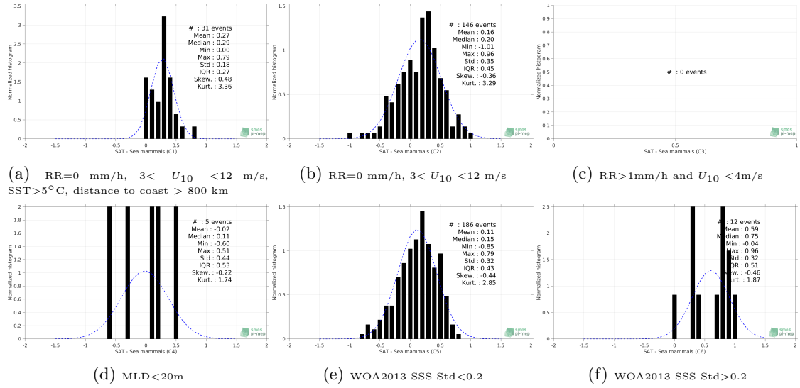
Figure 13: Normalized histogram of \Delta SSS (SMOS L3 v317 - 10 Days - 25 km (CATDS-CPDC) - Sea mammals) for 6 different subdatasets corresponding to: RR=0 mm/h, 3 < U_{10} < 12 m/s, SST>5°C, distance to coast > 800 km (a), RR=0 mm/h, 3 < U_{10} < 12 m/s (b), RR>1mm/h and U_{10} < 4 m/s (c), MLD<20m (d), WOA2013 SSS Std<0.2 (e), WOA2013 SSS Std>0.2 (f).
