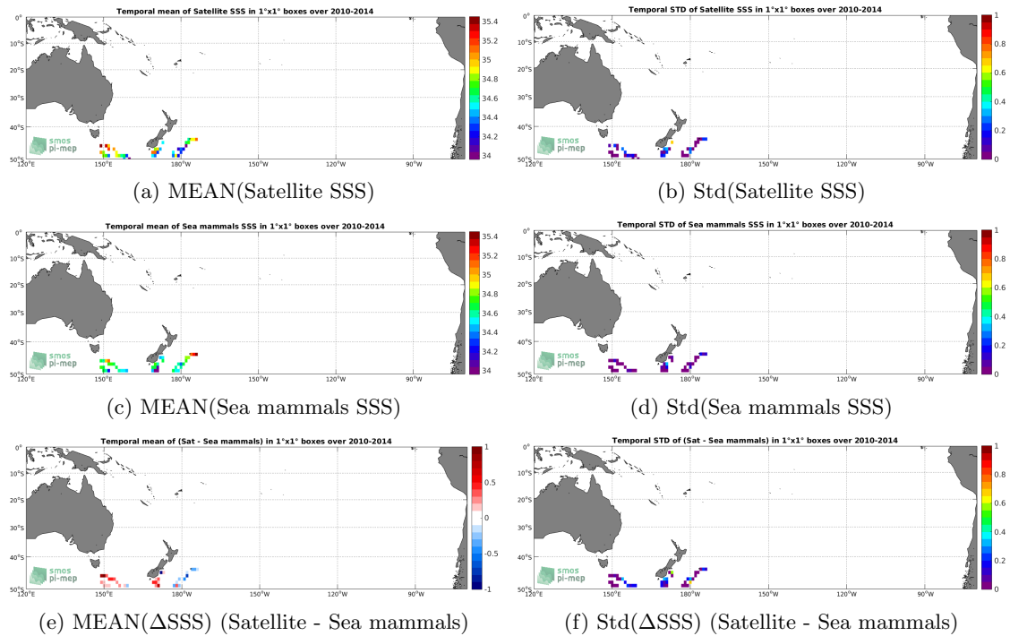
Figure 6: Temporal mean (left) and Std (right) of SSS from SMOS L3 v317 - 10 Days - 25 km (CATDS-CPDC) (top), Sea mammals (middle), and of \Delta SSS (Satellite - Sea mammals). Only match-up pairs are used to generate these maps.
