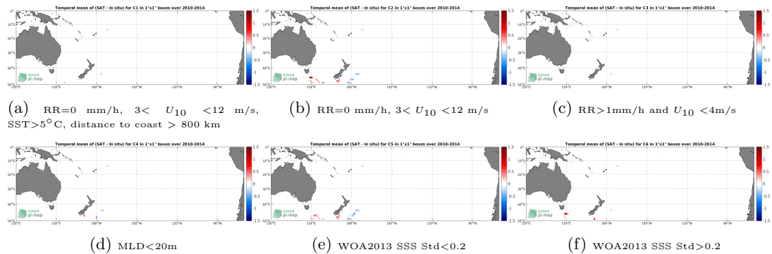
Figure 12: Temporal mean gridded over spatial boxes of size 1^{\circ}\times 1^{\circ} of \Delta\text{SSS} (SMOS L3 v317 - 10 Days - 25 km (CATDS-CPDC) - Sea mammals) for 6 different subdatasets corresponding to:RR=0 mm/h, 3 < U_{10} < 12 m/s, SST >5^{\circ}\text{C} , distance to coast > 800 km (a), RR=0 mm/h, 3 < U_{10} < 12 m/s (b), RR >1\text{mm/h} and U_{10} < 4\text{m/s} (c),MLD <20\text{m} (d),WOA2013 SSS Std <0.2 (e),WOA2013 SSS Std >0.2 (f).
