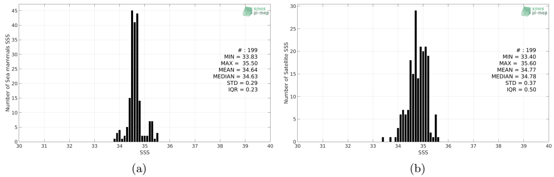
Figure 2: Histograms of SSS from Sea mammals (a) and SMOS L3 v317 - 10 Days - 25 km (CATDS-CPDC) (b) considering all match-up pairs per bins of 0.1 over the South Pacific Ocean Pi-MEP region and for the full satellite product period.
