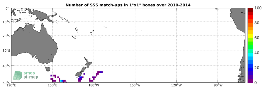
Figure 4: Number of SSS match-ups between Sea mammals SSS and the SMOS L3 v317 - 10 Days - 25 km (CATDS-CPDC) SSS product for the South Pacific Ocean Pi-MEP region over 1^\circ \times 1^\circ boxes and for the full satellite product period.
