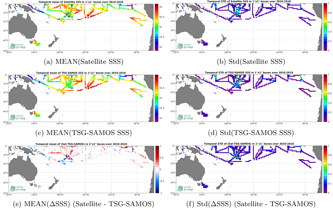
Figure 6: Temporal mean (left) and Std (right) of SSS from SMOS-L3-CATDS-CPDC-V3-MONTHLY-25KM (top), TSG-SAMOS (middle), and of \Delta SSS (Satellite - TSG-SAMOS). Only match-up pairs are used to generate these maps.
