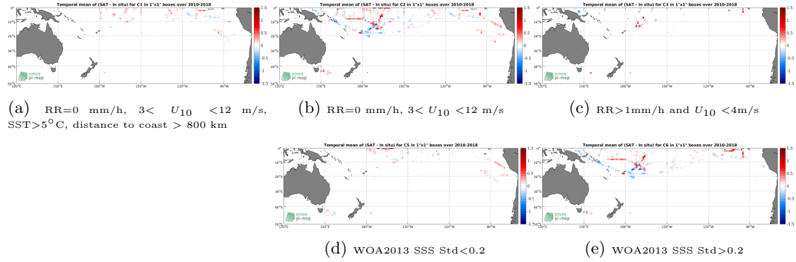
Figure 12: Temporal mean gridded over spatial boxes of size 1^\circ \times 1^\circ of \Delta SSS (SMOS-L3-CATDS-CPDC-V3-MONTHLY-25KM - TSG-SAMOS) for 5 different subdatasets corresponding to: RR=0 mm/h, 3 < U_{10} < 12 m/s, SST > 5^\circ\text{C} , distance to coast > 800 km (a), RR=0 mm/h, 3 < U_{10} < 12 m/s (b), RR > 1 mm/h and U_{10} < 4 m/s (c), WOA2013 SSS Std < 0.2 (d), WOA2013 SSS Std > 0.2 (e).
