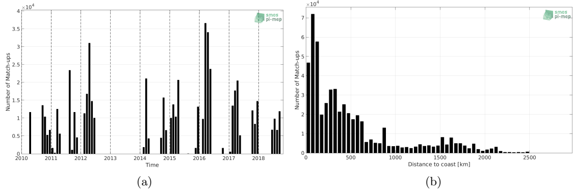
Figure 1: Number of match-ups between TSG-SAMOS and SMOS-L3-CATDS-CPDC-V3-MONTHLY-25KM SSS as a function of time (a) and as function of the distance to coast (b) over the South Pacific Ocean Pi-MEP region and for the full satellite product period.
