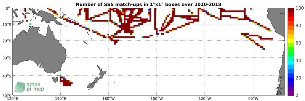
Figure 4: Number of SSS match-ups between TSG-SAMOS SSS and the SMOS-L3-CATDS-CPDC-V3-MONTHLY-25KM SSS product for the South Pacific Ocean Pi-MEP region over 1^\circ \times 1^\circ boxes and for the full satellite product period.
