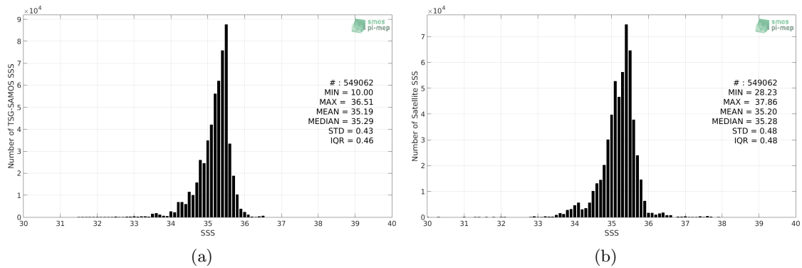
Figure 2: Histograms of SSS from TSG-SAMOS (a) and SMOS-L3-CATDS-CPDC-V3-MONTHLY-25KM (b) considering all match-up pairs per bins of 0.1 over the South Pacific Ocean Pi-MEP region and for the full satellite product period.
