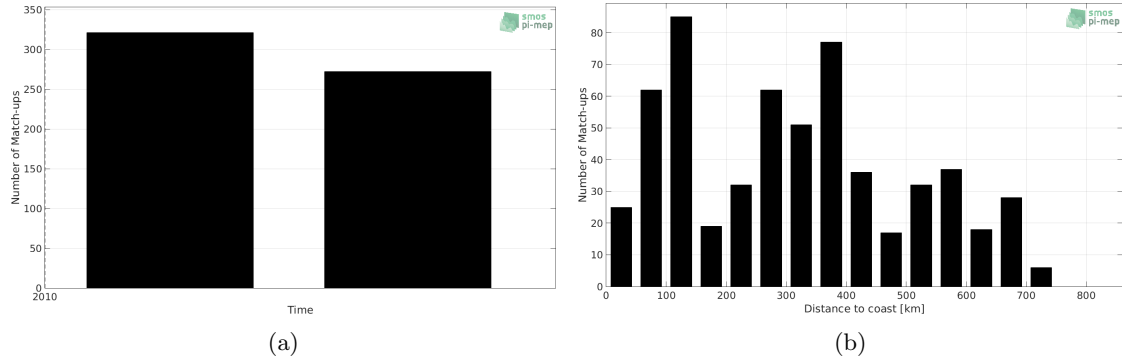
Figure 1: Number of match-ups between TSG-POLARSTERN and SMOS-L3-CATDS-CPDC-V3-MONTHLY-25KM SSS as a function of time (a) and as function of the distance to coast (b) over the South Pacific Ocean Pi-MEP region and for the full satellite product period.
