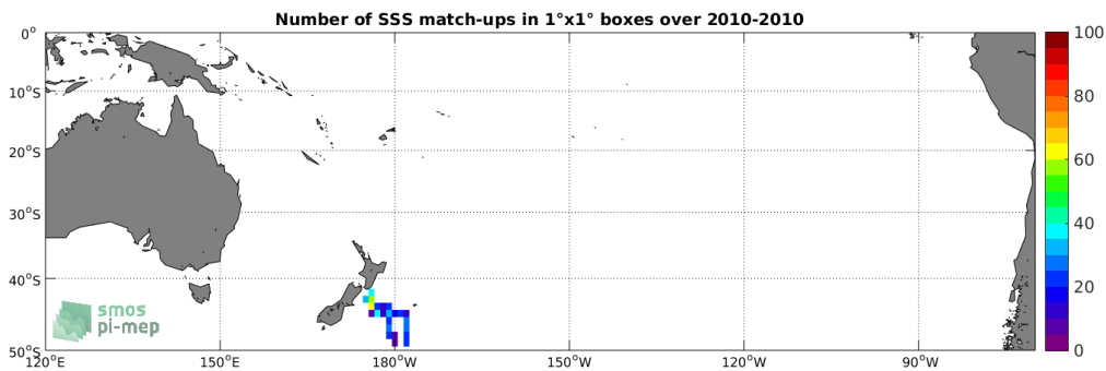
Figure 4: Number of SSS match-ups between TSG-POLARSTERN SSS and the SMOS-L3-CATDS-CPDC-V3-MONTHLY-25KM SSS product for the South Pacific Ocean Pi-MEP region over 1^\circ \times 1^\circ boxes and for the full satellite product period.
