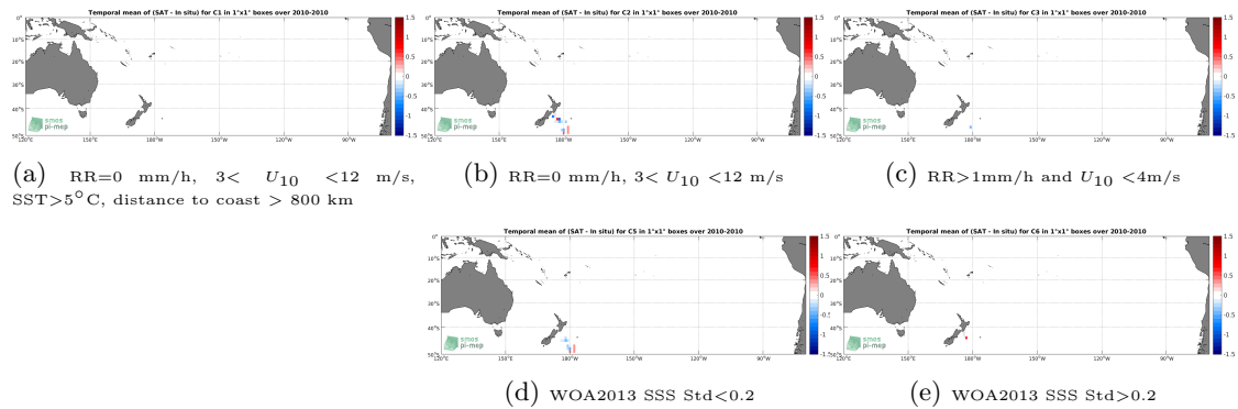
Figure 12: Temporal mean gridded over spatial boxes of size 1^\circ \times 1^\circ of \Delta SSS (SMOS-L3-CATDS-CPDC-V3-MONTHLY-25KM - TSG-POLARSTERN) for 5 different subdatasets corresponding to:RR=0 mm/h, 3 < U_{10} < 12 m/s, SST >5^\circ C, distance to coast > 800 km (a), RR=0 mm/h, 3 < U_{10} < 12 m/s (b), RR >1 mm/h and U_{10} < 4 m/s (c), WOA2013 SSS Std <0.2 (d), WOA2013 SSS Std >0.2 (e).
