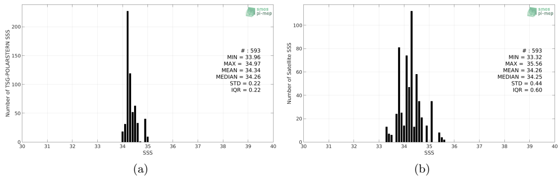
Figure 2: Histograms of SSS from TSG-POLARSTERN (a) and SMOS-L3-CATDS-CPDC-V3-MONTHLY-25KM (b) considering all match-up pairs per bins of 0.1 over the South Pacific Ocean Pi-MEP region and for the full satellite product period.
