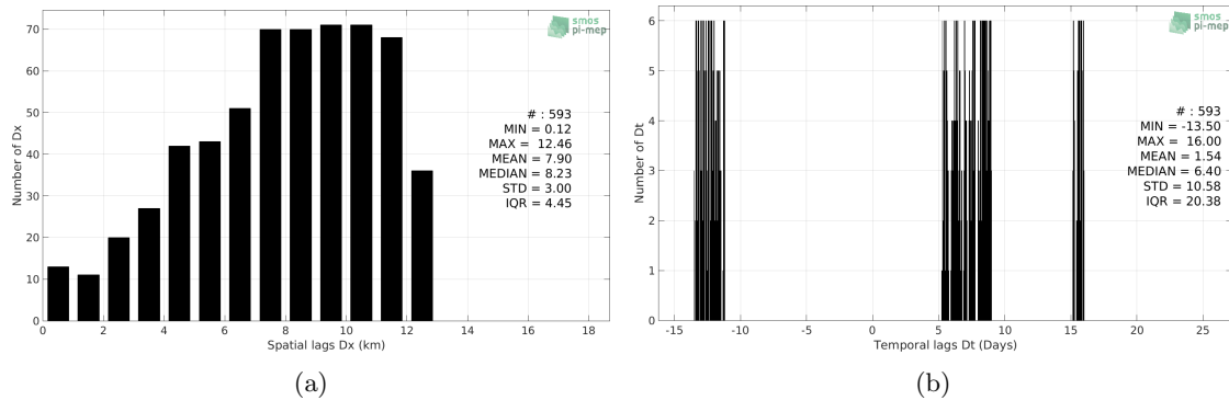
Figure 5: Histograms of the spatial (a) and temporal (b) lags between the time of the TSG-POLARSTERN measurements and the date of the corresponding SMOS-L3-CATDS-CPDC-V3-MONTHLY-25KM SSS product.
