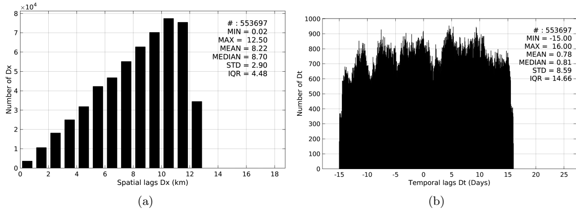
Figure 5: Histograms of the spatial (a) and temporal (b) lags between the time of the TSG-LEGOS-DM measurements and the date of the corresponding SMOS-L3-CATDS-CPDC-V3-MONTHLY-25KM SSS product.
