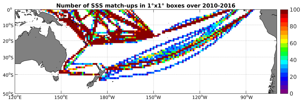
Figure 4: Number of SSS match-ups between TSG-LEGOS-DM SSS and the SMOS-L3-CATDS-CPDC-V3-MONTHLY-25KM SSS product for the South Pacific Ocean Pi-MEP region over 1°x1° boxes and for the full satellite product period.
