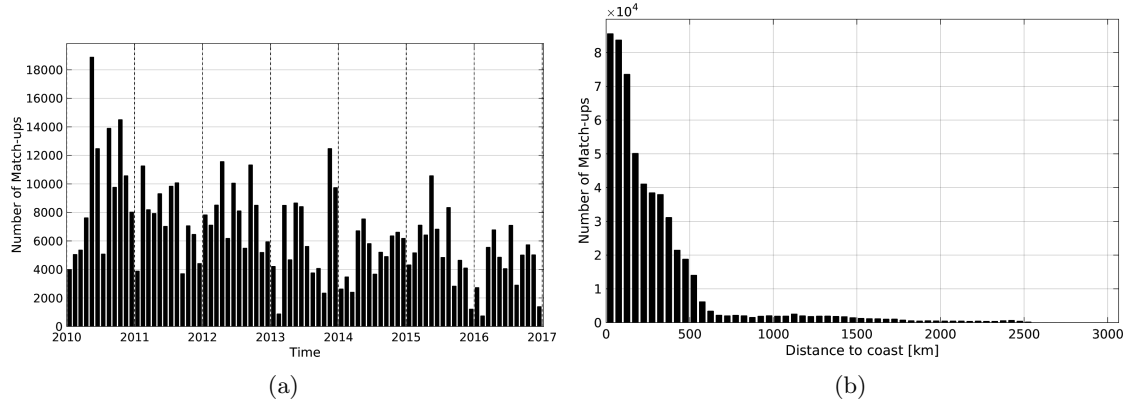
Figure 1: Number of match-ups between TSG-LEGOS-DM and SMOS-L3-CATDS-CPDC-V3-MONTHLY-25KM SSS as a function of time (a) and as function of the distance to coast (b) over the South Pacific Ocean Pi-MEP region and for the full satellite product period.
