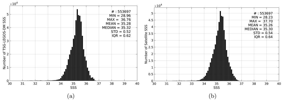
Figure 2: Histograms of SSS from TSG-LEGOS-DM (a) and SMOS-L3-CATDS-CPDC-V3-MONTHLY-25KM (b) considering all match-up pairs per bins of 0.1 over the South Pacific Ocean Pi-MEP region and for the full satellite product period.
