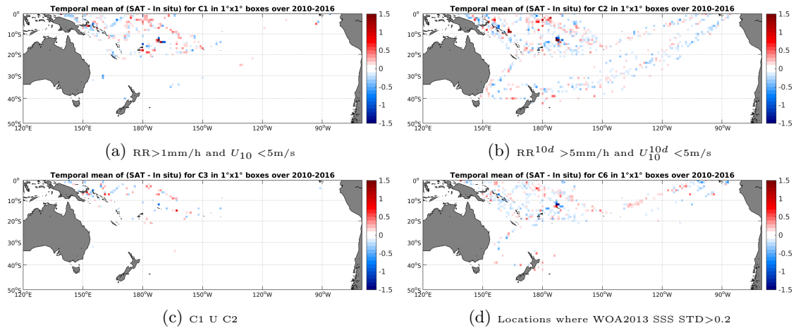
Figure 12: Temporal mean gridded over spatial boxes of size 1^\circ \times 1^\circ of \Delta SSS (SMOS-L3-CATDS-CPDC-V3-MONTHLY-25KM - TSG-LEGOS-DM) for 4 different subdatasets corresponding to: RR > 1mm/h and U_{10} < 5 m/s (a), RR^{10d} > 5 mm/h and U_{10}^{10d} < 5 m/s (b), C1 U C2 (c), Locations where WOA2013 SSS STD > 0.2 (d).
