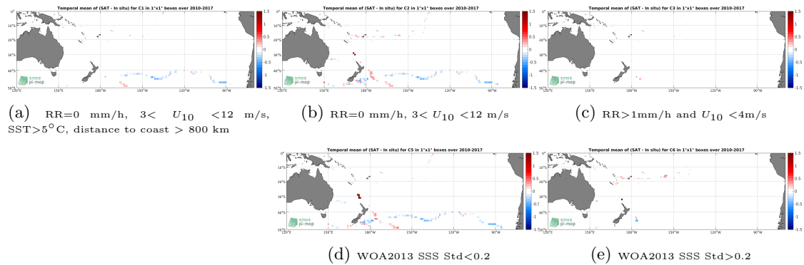
Figure 12: Temporal mean gridded over spatial boxes of size 1^\circ \times 1^\circ of \Delta SSS (SMOS-L3-CATDS-CPDC-V3-MONTHLY-25KM - TSG-GOSUD-Sailing-ship) for 5 different subdatasets corresponding to:RR=0 mm/h, 3 < U_{10} < 12 m/s, SST >5^\circ C, distance to coast > 800 km (a), RR=0 mm/h, 3 < U_{10} < 12 m/s (b), RR >1 mm/h and U_{10} < 4 m/s (c), WOA2013 SSS Std <0.2 (d), WOA2013 SSS Std >0.2 (e).
