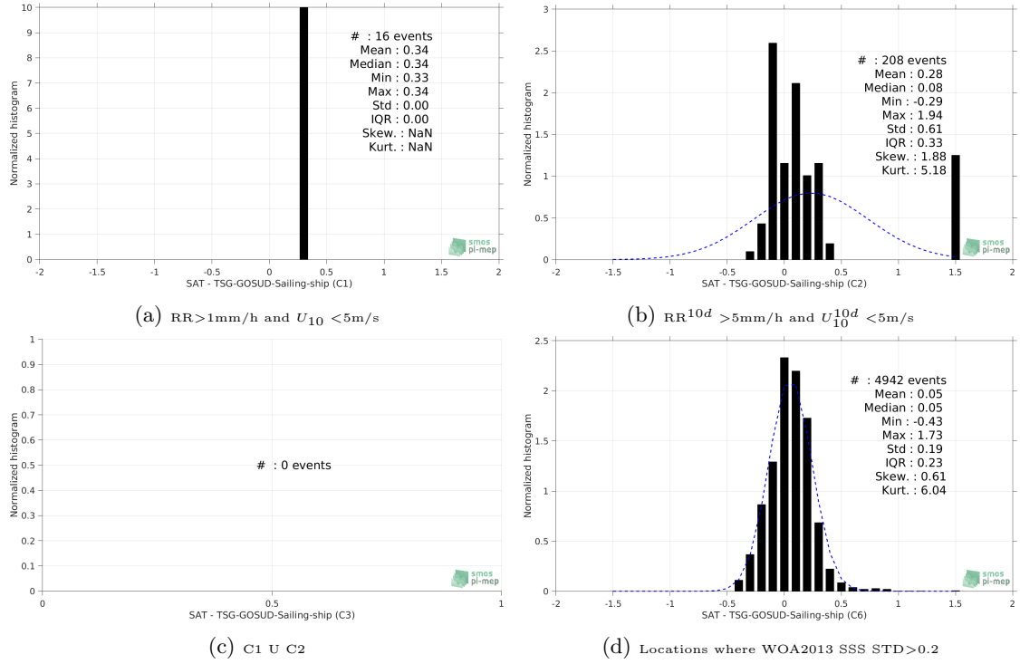
Figure 13: Normalized histogram of \Delta\text{SSS} (SMOS-L3-CATDS-CPDC-V3-MONTHLY-25KM - TSG-GOSUD-Sailing-ship) for 6 different subdatasets corresponding to: RR > 1\text{mm/h} and U_{10} < 5\text{m/s} (a), RR^{10d} > 5\text{mm/h} and U_{10}^{10d} < 5\text{m/s} (b), C1 U C2 (c), Locations where WOA2013 SSS STD > 0.2 (d).
