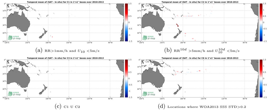
Figure 12: Temporal mean gridded over spatial boxes of size 1^\circ \times 1^\circ of \Delta SSS (SMOS-L3-CATDS-CPDC-V3-MONTHLY-25KM - TSG-GOSUD-Sailing-ship) for 4 different subdatasets corresponding to:RR >1 mm/h and U_{10} < 5 m/s (a), RR ^{10d} > 5 mm/h and U_{10}^{10d} < 5 m/s (b), C1 U C2 (c),Locations where WOA2013 SSS STD >0.2 (d).
