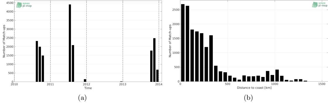
Figure 1: Number of match-ups between TSG-GOSUD-Sailing-ship and SMOS-L3-CATDS-CPDC-V3-MONTHLY-25KM SSS as a function of time (a) and as function of the distance to coast (b) over the South Pacific Ocean Pi-MEP region and for the full satellite product period.
