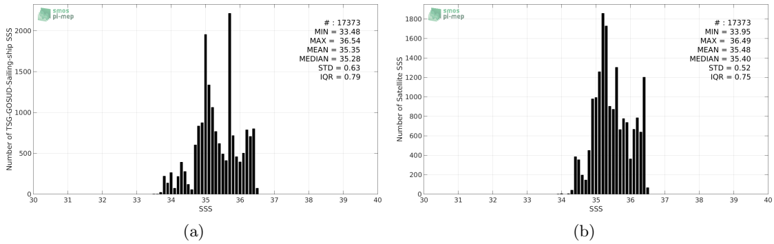
Figure 2: Histograms of SSS from TSG-GOSUD-Sailing-ship (a) and SMOS-L3-CATDS-CPDC-V3-MONTHLY-25KM (b) considering all match-up pairs per bins of 0.1 over the South Pacific Ocean Pi-MEP region and for the full satellite product period.
