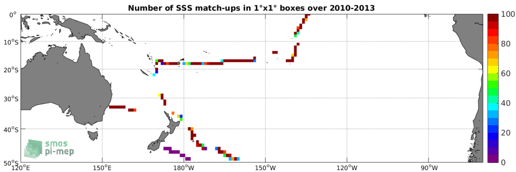
Figure 4: Number of SSS match-ups between TSG-GOSUD-Sailing-ship SSS and the SMOS-L3-CATDS-CPDC-V3-MONTHLY-25KM SSS product for the South Pacific Ocean Pi-MEP region over 1^\circ \times 1^\circ boxes and for the full satellite product period.
