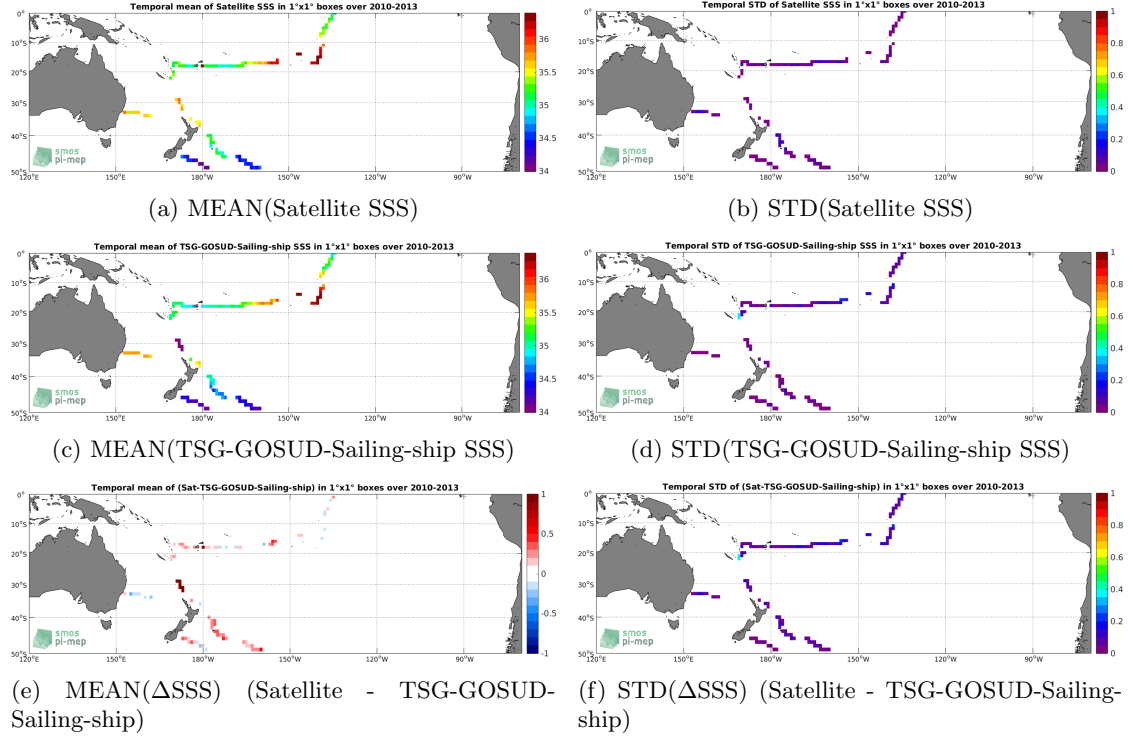
Figure 6: Temporal mean (left) and STD (right) of SSS from SMOS-L3-CATDS-CPDC-V3-MONTHLY-25KM (top), TSG-GOSUD-Sailing-ship (middle), and of \Delta SSS (Satellite - TSG-GOSUD-Sailing-ship). Only match-up pairs are used to generate these maps.
