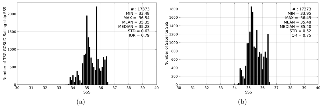
Figure 2: Histograms of SSS from TSG-GOSUD-Sailing-ship (a) and SMOS-L3-CATDS-CPDC-V3-MONTHLY-25KM (b) considering all match-up pairs per bins of 0.1 over the South Pacific Ocean Pi-MEP region and for the full satellite product period.
