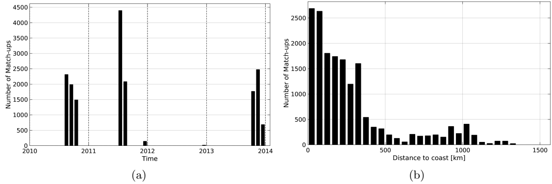
Figure 1: Number of match-ups between TSG-GOSUD-Sailing-ship and SMOS-L3-CATDS-CPDC-V3-MONTHLY-25KM SSS as a function of time (a) and as function of the distance to coast (b) over the South Pacific Ocean Pi-MEP region and for the full satellite product period.
