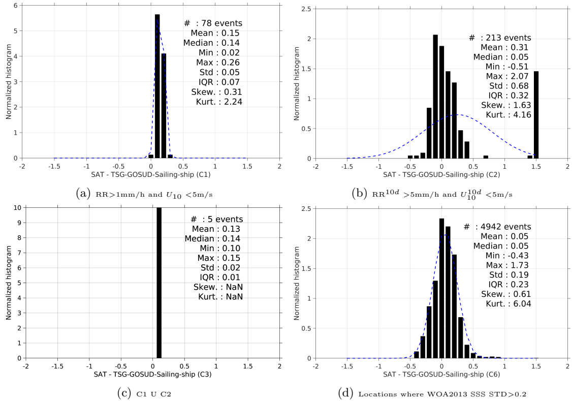
Figure 13: Normalized histogram of \Delta\text{SSS} (SMOS-L3-CATDS-CPDC-V3-MONTHLY-25KM - TSG-GOSUD-Sailing-ship) for 6 different subdatasets corresponding to: RR > 1mm/h and U_{10} < 5\text{m/s} (a), RR^{10d} > 5\text{mm/h} and U_{10}^{10d} < 5\text{m/s} (b), C1 U C2 (c), Locations where WOA2013 SSS STD > 0.2 (d).
