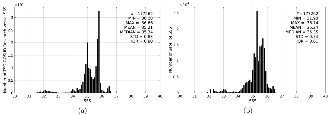
Figure 2: Histograms of SSS from TSG-GOSUD-Research-vessel (a) and SMOS-L3-CATDS-CPDC-V3-MONTHLY-25KM (b) considering all match-up pairs per bins of 0.1 over the South Pacific Ocean Pi-MEP region and for the full satellite product period.
