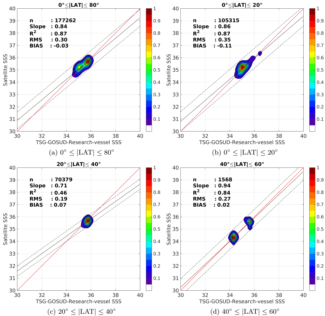
Figure 9: Contour maps of the concentration of SMOS-L3-CATDS-CPDC-V3-MONTHLY-25KM SSS (y-axis) versus TSG-GOSUD-Research-vessel SSS (x-axis) at match-up pairs for different latitude bands. For each plot, the red line shows x=y . The black thin and dashed lines indicate a linear fit through the data cloud and the \pm 95\% confidence levels, respectively. The number of match-up pairs n , the slope and R^2 coefficient of the linear fit, the root mean square (RMS) and the mean bias between satellite and in situ data are indicated for each latitude band in each plot.
