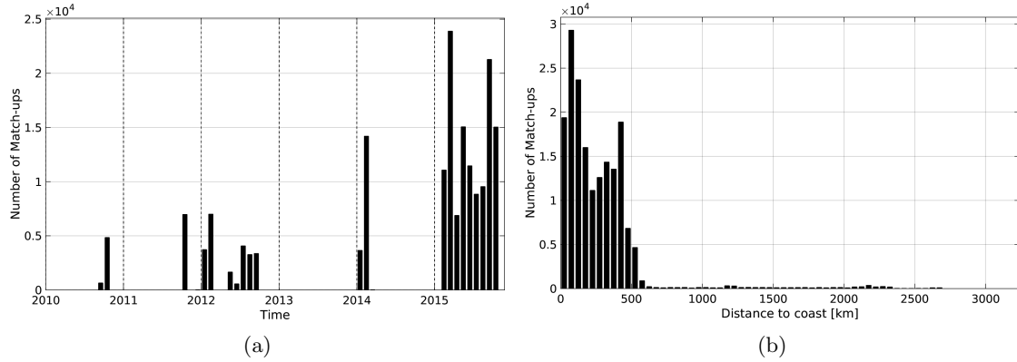
Figure 1: Number of match-ups between TSG-GOSUD-Research-vessel and SMOS-L3-CATDS-CPDC-V3-MONTHLY-25KM SSS as a function of time (a) and as function of the distance to coast (b) over the South Pacific Ocean Pi-MEP region and for the full satellite product period.
