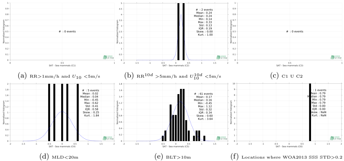
Figure 13: Normalized histogram of \Delta SSS (SMOS-L3-CATDS-CPDC-V3-MONTHLY-25KM - Sea mammals) for 6 different subdatasets corresponding to: RR>1mm/h and U_{10} <5m/s (a), RR^{10d} >5mm/h and U_{10}^{10d} <5m/s (b), C1 U C2 (c),MLD<20m (d),BLT>10m (e),Locations where WOA2013 SSS STD>0.2 (f).
