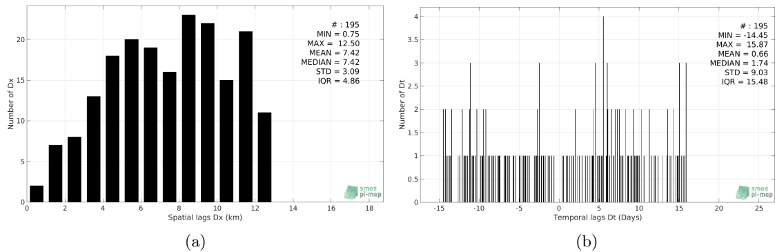
Figure 5: Histograms of the spatial (a) and temporal (b) lags between the time of the Sea mammals measurements and the date of the corresponding SMOS-L3-CATDS-CPDC-V3-MONTHLY-25KM SSS product.
