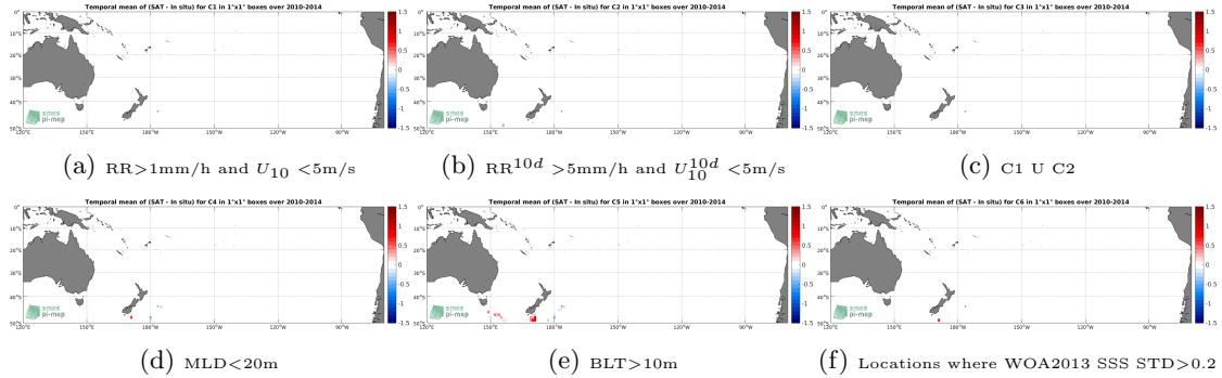
Figure 12: Temporal mean gridded over spatial boxes of size 1°x1° of \Delta SSS (SMOS-L3-CATDS-CPDC-V3-MONTHLY-25KM - Sea mammals) for 6 different subdatasets corresponding to:RR>1mm/h and U_{10} <5m/s (a), RR^{10d} >5mm/h and U_{10}^{10d} <5m/s (b), C1 U C2 (c),MLD<20m (d),BLT>10m (e),Locations where WOA2013 SSS STD>0.2 (f).
