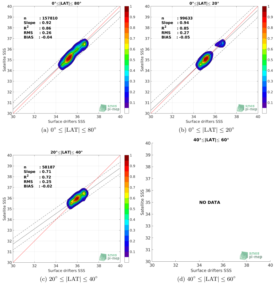
Figure 8: Contour maps of the concentration of SMOS-L3-CATDS-CPDC-V3-MONTHLY-25KM SSS (y-axis) versus Surface drifters SSS (x-axis) at match-up pairs for different latitude bands. For each plot, the red line shows x=y . The black thin and dashed lines indicate a linear fit through the data cloud and the \pm 95\% confidence levels, respectively. The number match-up pairs n , the slope and R^2 coefficient of the linear fit, the root mean square (RMS) and the mean bias between satellite and in situ data are indicated for each latitude band in each plots.
