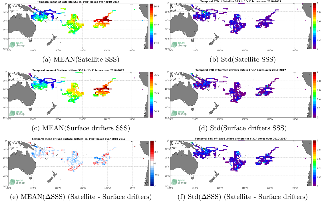
Figure 5: Temporal mean (left) and Std (right) of SSS from SMOS-L3-CATDS-CPDC-V3-MONTHLY-25KM (top), Surface drifters (middle), and of \Delta SSS (Satellite - Surface drifters). Only match-up pairs are used to generate these maps.
