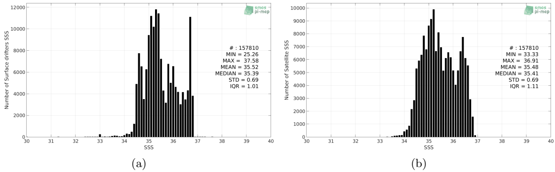
Figure 2: Histograms of SSS from Surface drifters (a) and SMOS-L3-CATDS-CPDC-V3-MONTHLY-25KM (b) considering all match-up pairs per bins of 0.1 over the South Pacific Ocean Pi-MEP region and for the full satellite product period.
