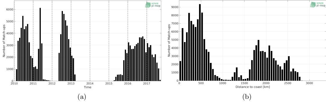
Figure 1: Number of match-ups between Surface drifters and SMOS-L3-CATDS-CPDC-V3-MONTHLY-25KM SSS as a function of time (a) and as function of the distance to coast (b) over the South Pacific Ocean Pi-MEP region and for the full satellite product period.
