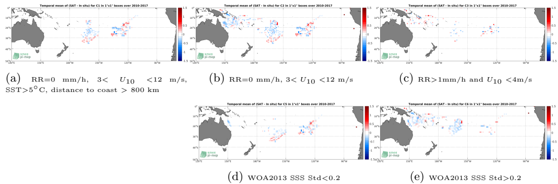
Figure 11: Temporal mean gridded over spatial boxes of size 1^\circ \times 1^\circ of \Delta SSS (SMOS-L3-CATDS-CPDC-V3-MONTHLY-25KM - Surface drifters) for 5 different subdatasets corresponding to:RR=0 mm/h, 3 < U_{10} < 12 m/s, SST >5^\circ C, distance to coast > 800 km (a), RR=0 mm/h, 3 < U_{10} < 12 m/s (b), RR >1 mm/h and U_{10} < 4 m/s (c), WOA2013 SSS Std <0.2 (d), WOA2013 SSS Std >0.2 (e).
