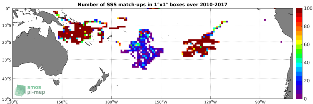
Figure 3: Number of SSS match-ups between Surface drifters SSS and the SMOS-L3-CATDS-CPDC-V3-MONTHLY-25KM SSS product for the South Pacific Ocean Pi-MEP region over 1^\circ \times 1^\circ boxes and for the full satellite product period.
