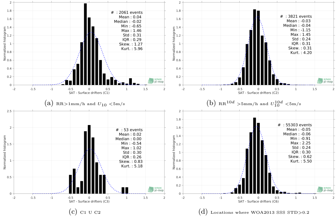
Figure 12: Normalized histogram of \Delta\text{SSS} (SMOS-L3-CATDS-CPDC-V3-MONTHLY-25KM - Surface drifters) for 6 different subdatasets corresponding to: RR > 1mm/h and U_{10} < 5\text{m/s} (a), RR^{10d} > 5\text{mm/h} and U_{10}^{10d} < 5\text{m/s} (b), C1 U C2 (c), Locations where WOA2013 SSS STD > 0.2 (d).
