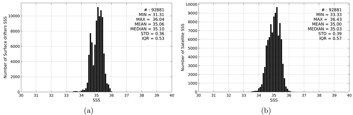
Figure 2: Histograms of SSS from Surface drifters (a) and SMOS-L3-CATDS-CPDC-V3-MONTHLY-25KM (b) considering all match-up pairs per bins of 0.1 over the South Pacific Ocean Pi-MEP region and for the full satellite product period.
