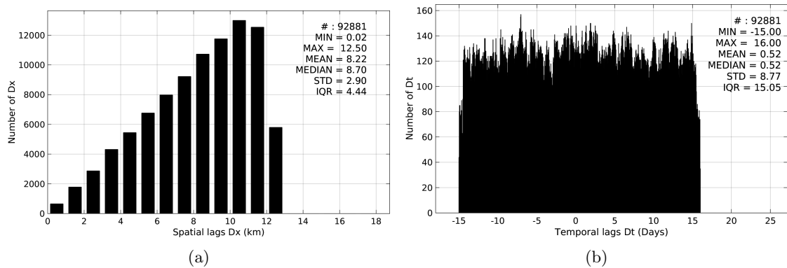
Figure 4: Histograms of the spatial (a) and temporal (b) lags between the time of the Surface drifters measurements and the date of the corresponding SMOS-L3-CATDS-CPDC-V3-MONTHLY-25KM SSS product.
