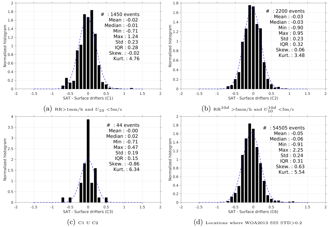
Figure 12: Normalized histogram of \Delta\text{SSS} (SMOS-L3-CATDS-CPDC-V3-MONTHLY-25KM - Surface drifters) for 6 different subdatasets corresponding to: RR>1mm/h and U_{10} < 5\text{m/s} (a), RR^{10d} > 5\text{mm/h} and U_{10}^{10d} < 5\text{m/s} (b), C1 U C2 (c), Locations where WOA2013 SSS STD>0.2 (d).
