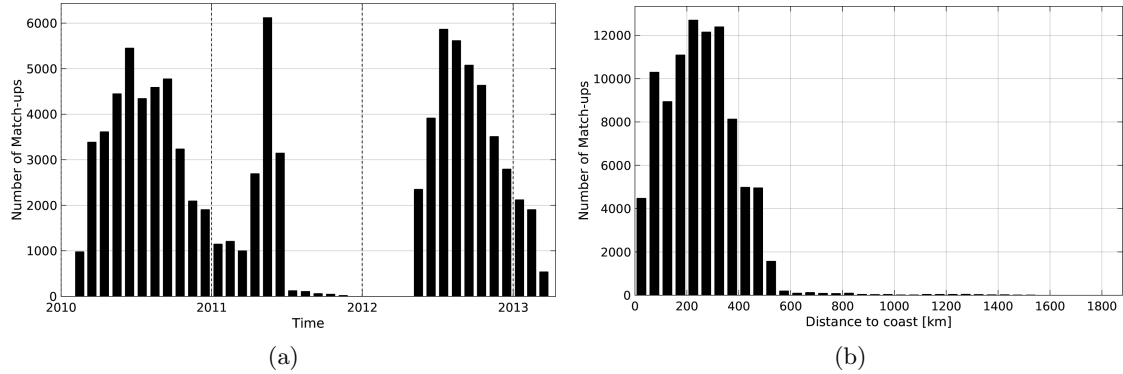
Figure 1: Number of match-ups between Surface drifters and SMOS-L3-CATDS-CPDC-V3-MONTHLY-25KM SSS as a function of time (a) and as function of the distance to coast (b) over the South Pacific Ocean Pi-MEP region and for the full satellite product period.
