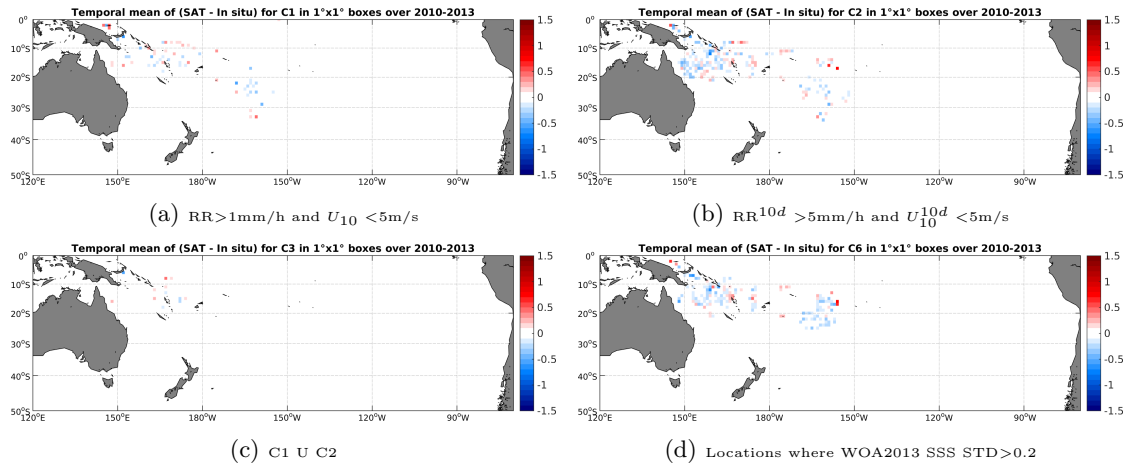
Figure 11: Temporal mean gridded over spatial boxes of size 1^\circ \times 1^\circ of \Delta SSS (SMOS-L3-CATDS-CPDC-V3-MONTHLY-25KM - Surface drifters) for 4 different subdatasets corresponding to: RR > 1 mm/h and U_{10} < 5 m/s (a), RR 10d > 5 mm/h and U_{10}^{10d} < 5 m/s (b), C1 U C2 (c), Locations where WOA2013 SSS STD > 0.2 (d).
