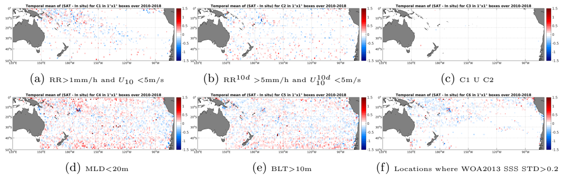
Figure 12: Temporal mean gridded over spatial boxes of size 1^\circ \times 1^\circ of \Delta SSS (SMOS-L3-CATDS-CPDC-V3-MONTHLY-25KM - Argo) for 6 different subdatasets corresponding to:RR >1 mm/h and U_{10} < 5 m/s (a), RR^{10d} > 5 mm/h and U_{10}^{10d} < 5 m/s (b), C1 U C2 (c),MLD <20 m (d),BLT >10 m (e),Locations where WOA2013 SSS STD >0.2 (f).
