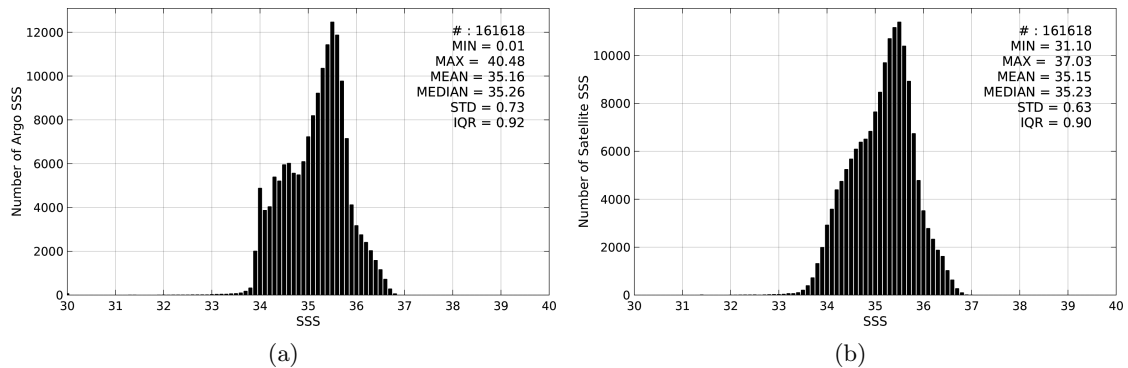
Figure 2: Histograms of SSS from Argo (a) and SMOS-L3-CATDS-CPDC-V3-MONTHLY-25KM (b) considering all match-up pairs per bins of 0.1 over the South Pacific Ocean Pi-MEP region and for the full satellite product period.
