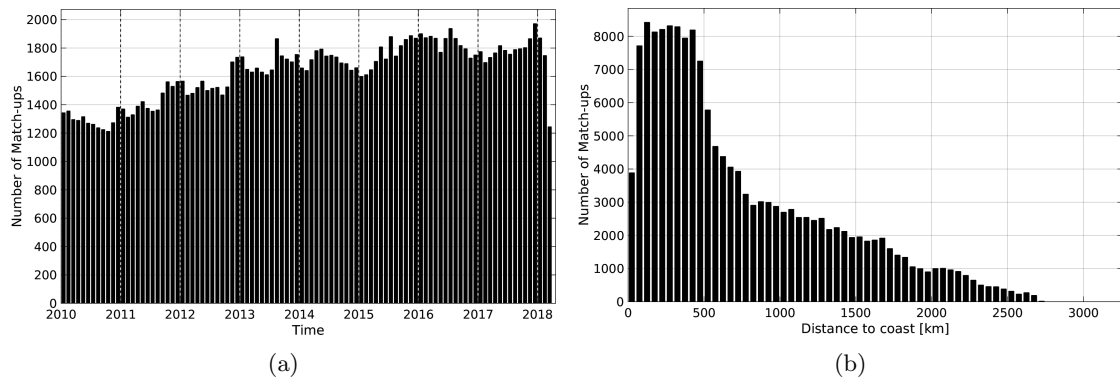
Figure 1: Number of match-ups between Argo and SMOS-L3-CATDS-CPDC-V3-MONTHLY-25KM SSS as a function of time (a) and as function of the distance to coast (b) over the South Pacific Ocean Pi-MEP region and for the full satellite product period.
