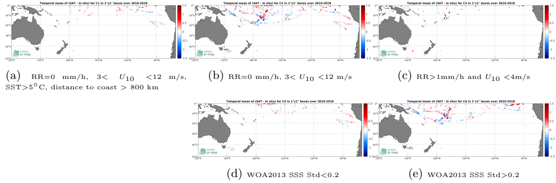
Figure 12: Temporal mean gridded over spatial boxes of size 1^\circ \times 1^\circ of \Delta SSS (SMOS-L3-CATDS-CPDC-V3-10DAYS-25KM - TSG-SAMOS) for 5 different subdatasets corresponding to: RR=0 mm/h, 3 < U_{10} < 12 m/s, SST > 5^\circ\text{C} , distance to coast > 800 km (a), RR=0 mm/h, 3 < U_{10} < 12 m/s (b), RR > 1 mm/h and U_{10} < 4 m/s (c), WOA2013 SSS Std < 0.2 (d), WOA2013 SSS Std > 0.2 (e).
