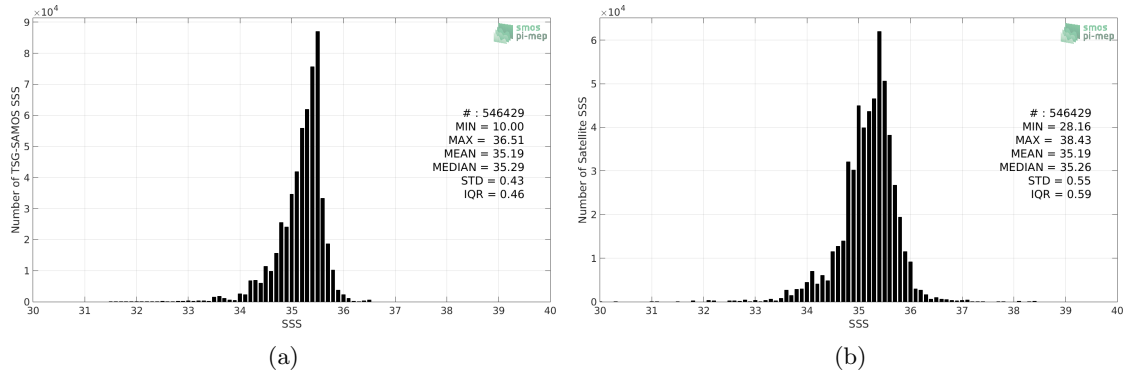
Figure 2: Histograms of SSS from TSG-SAMOS (a) and SMOS-L3-CATDS-CPDC-V3-10DAYS-25KM (b) considering all match-up pairs per bins of 0.1 over the South Pacific Ocean Pi-MEP region and for the full satellite product period.
