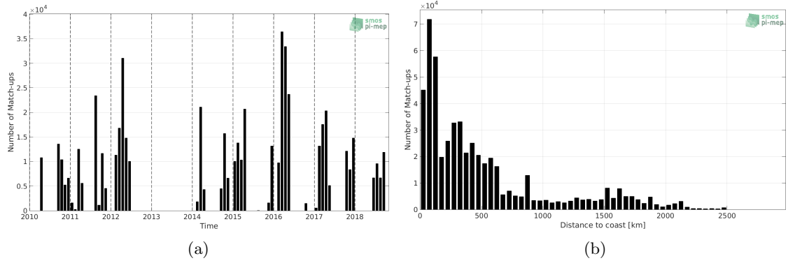
Figure 1: Number of match-ups between TSG-SAMOS and SMOS-L3-CATDS-CPDC-V3-10DAYS-25KM SSS as a function of time (a) and as function of the distance to coast (b) over the South Pacific Ocean Pi-MEP region and for the full satellite product period.
