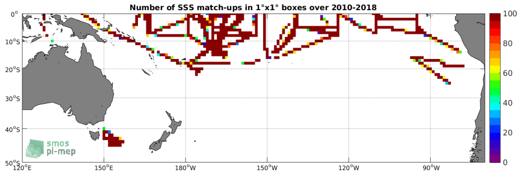
Figure 4: Number of SSS match-ups between TSG-SAMOS SSS and the SMOS-L3-CATDS-CPDC-V3-10DAYS-25KM SSS product for the South Pacific Ocean Pi-MEP region over 1^\circ \times 1^\circ boxes and for the full satellite product period.
