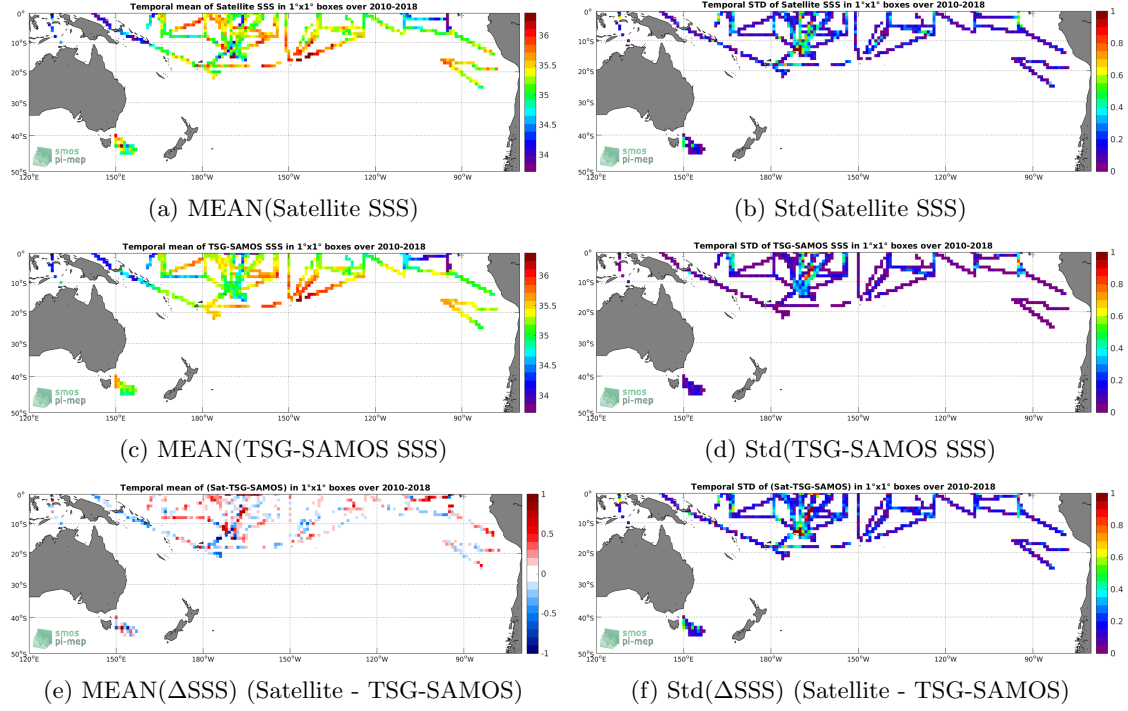
Figure 6: Temporal mean (left) and Std (right) of SSS from SMOS-L3-CATDS-CPDC-V3-10DAYS-25KM (top), TSG-SAMOS (middle), and of \Delta SSS (Satellite - TSG-SAMOS). Only match-up pairs are used to generate these maps.
