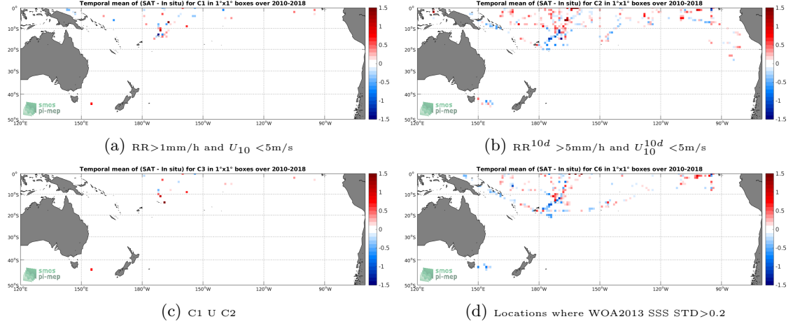
Figure 12: Temporal mean gridded over spatial boxes of size 1^\circ \times 1^\circ of \Delta SSS (SMOS-L3-CATDS-CPDC-V3-10DAYS-25KM - TSG-SAMOS) for 4 different subdatasets corresponding to: RR > 1mm/h and U_{10} < 5\text{m/s} (a), RR^{10d} > 5\text{mm/h} and U_{10}^{10d} < 5\text{m/s} (b), C1 U C2 (c), Locations where WOA2013 SSS STD > 0.2 (d).
