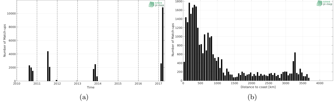
Figure 1: Number of match-ups between TSG-GOSUD-Sailing-ship and SMOS-L3-CATDS-CPDC-V3-10DAYS-25KM SSS as a function of time (a) and as function of the distance to coast (b) over the South Pacific Ocean Pi-MEP region and for the full satellite product period.
