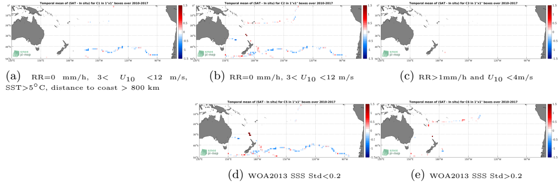
Figure 12: Temporal mean gridded over spatial boxes of size 1^\circ \times 1^\circ of \Delta SSS (SMOS-L3-CATDS-CPDC-V3-10DAYS-25KM - TSG-GOSUD-Sailing-ship) for 5 different subdatasets corresponding to: RR=0 mm/h, 3 < U_{10} < 12 m/s, SST > 5^\circ\text{C} , distance to coast > 800 km (a), RR=0 mm/h, 3 < U_{10} < 12 m/s (b), RR > 1 mm/h and U_{10} < 4 m/s (c), WOA2013 SSS Std < 0.2 (d), WOA2013 SSS Std > 0.2 (e).
