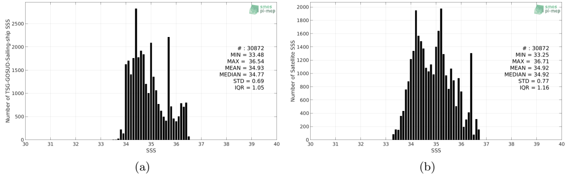
Figure 2: Histograms of SSS from TSG-GOSUD-Sailing-ship (a) and SMOS-L3-CATDS-CPDC-V3-10DAYS-25KM (b) considering all match-up pairs per bins of 0.1 over the South Pacific Ocean Pi-MEP region and for the full satellite product period.
