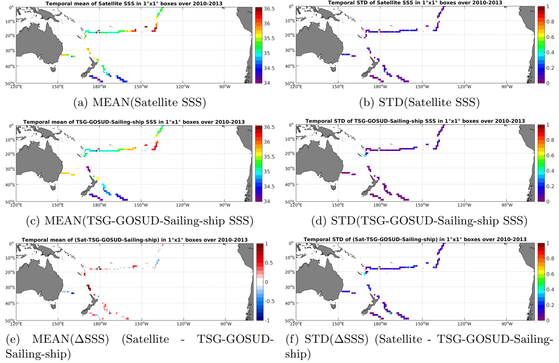
Figure 6: Temporal mean (left) and STD (right) of SSS from SMOS-L3-CATDS-CPDC-V3-10DAYS-25KM (top), TSG-GOSUD-Sailing-ship (middle), and of \Delta SSS (Satellite - TSG-GOSUD-Sailing-ship). Only match-up pairs are used to generate these maps.
