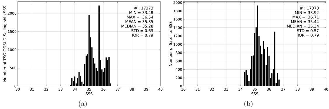
Figure 2: Histograms of SSS from TSG-GOSUD-Sailing-ship (a) and SMOS-L3-CATDS-CPDC-V3-10DAYS-25KM (b) considering all match-up pairs per bins of 0.1 over the South Pacific Ocean Pi-MEP region and for the full satellite product period.
