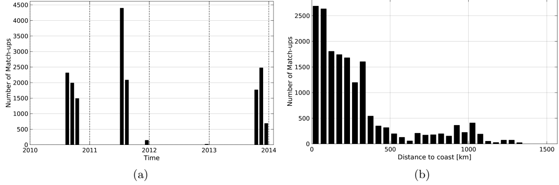
Figure 1: Number of match-ups between TSG-GOSUD-Sailing-ship and SMOS-L3-CATDS-CPDC-V3-10DAYS-25KM SSS as a function of time (a) and as function of the distance to coast (b) over the South Pacific Ocean Pi-MEP region and for the full satellite product period.
