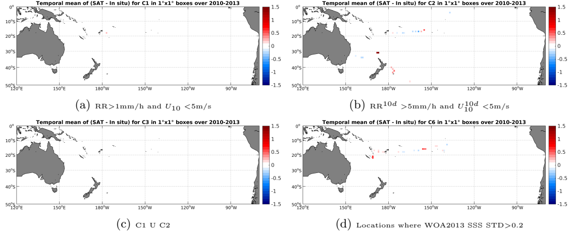
Figure 12: Temporal mean gridded over spatial boxes of size 1^\circ \times 1^\circ of \Delta SSS (SMOS-L3-CATDS-CPDC-V3-10DAYS-25KM - TSG-GOSUD-Sailing-ship) for 4 different subdatasets corresponding to: RR > 1 mm/h and U_{10} < 5 m/s (a), RR^{10d} > 5 mm/h and U_{10}^{10d} < 5 m/s (b), C1 U C2 (c), Locations where WOA2013 SSS STD > 0.2 (d).
