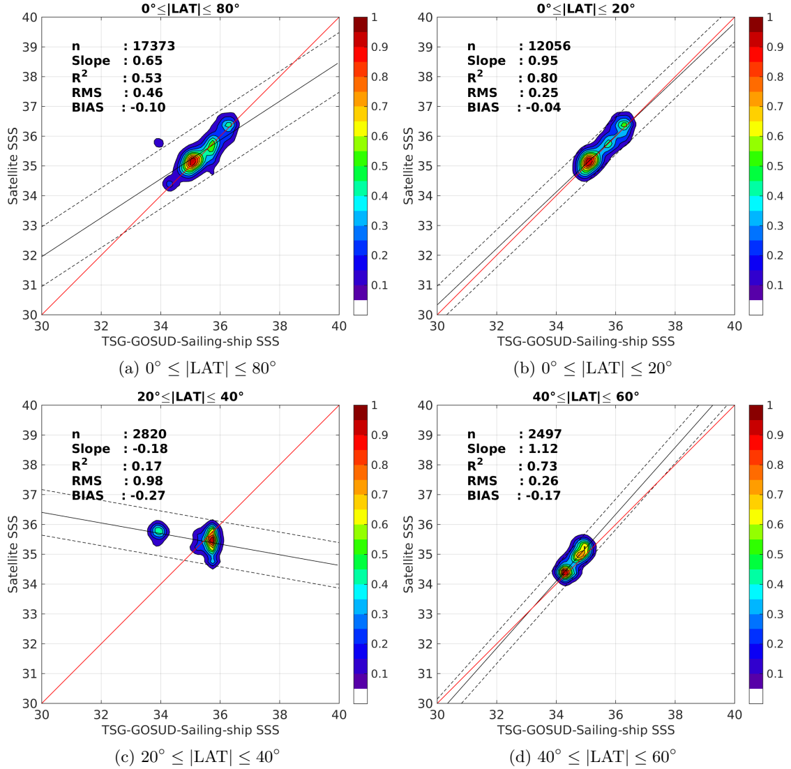
Figure 9: Contour maps of the concentration of SMOS-L3-CATDS-CPDC-V3-10DAYS-25KM SSS (y-axis) versus TSG-GOSUD-Sailing-ship SSS (x-axis) at match-up pairs for different latitude bands. For each plot, the red line shows x=y . The black thin and dashed lines indicate a linear fit through the data cloud and the \pm 95\% confidence levels, respectively. The number match-up pairs n , the slope and R^2 coefficient of the linear fit, the root mean square (RMS) and the mean bias between satellite and in situ data are indicated for each latitude band in each plots.
