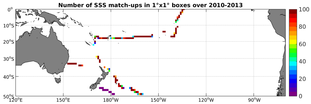
Figure 4: Number of SSS match-ups between TSG-GOSUD-Sailing-ship SSS and the SMOS-L3-CATDS-CPDC-V3-10DAYS-25KM SSS product for the South Pacific Ocean Pi-MEP region over 1^\circ \times 1^\circ boxes and for the full satellite product period.
