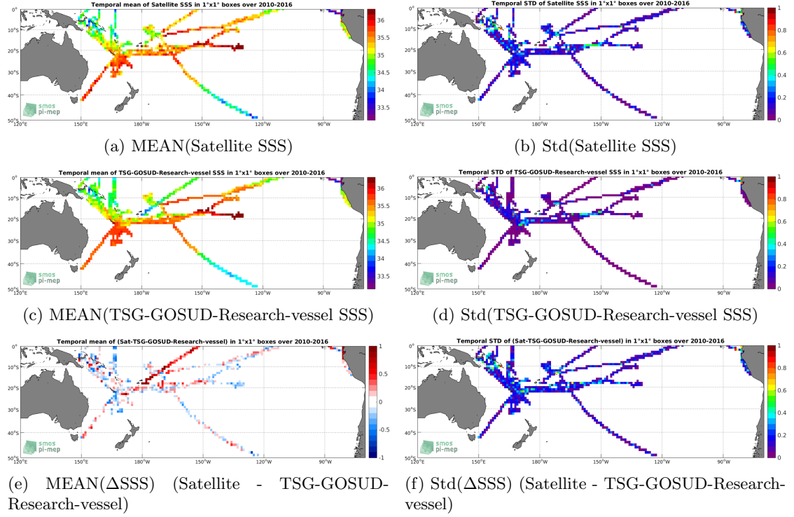
Figure 6: Temporal mean (left) and Std (right) of SSS from SMOS-L3-CATDS-CPDC-V3-10DAYS-25KM (top), TSG-GOSUD-Research-vessel (middle), and of \Delta SSS (Satellite - TSG-GOSUD-Research-vessel). Only match-up pairs are used to generate these maps.
