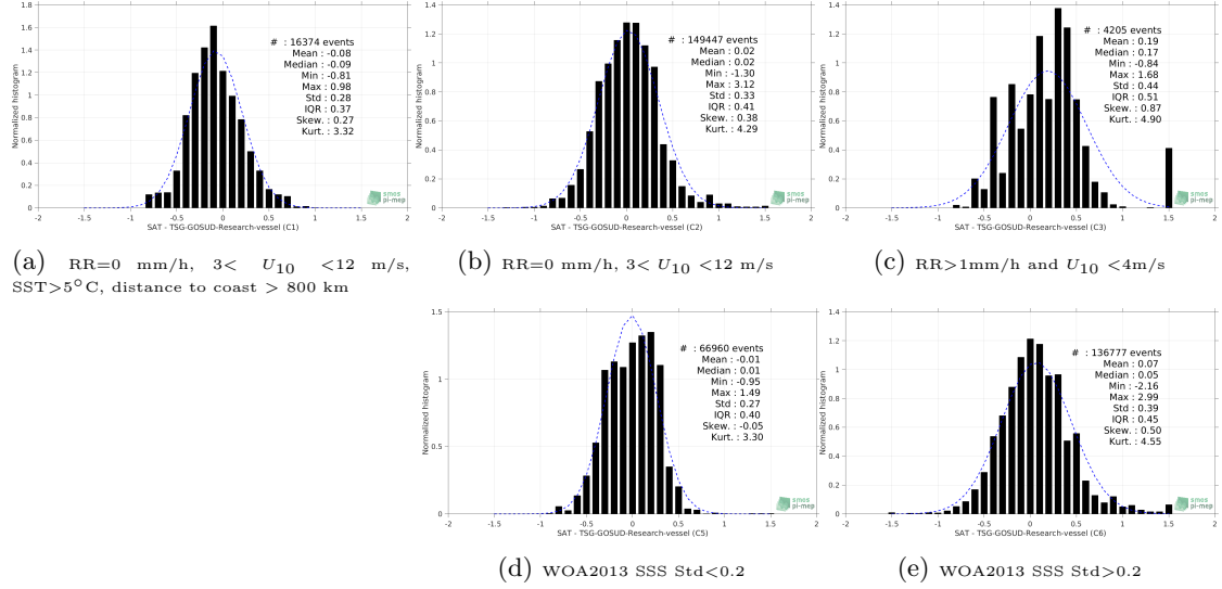
Figure 13: Normalized histogram of \Delta\text{SSS} (SMOS-L3-CATDS-CPDC-V3-10DAYS-25KM - TSG-GOSUD-Research-vessel) for 5 different subdatasets corresponding to: RR=0 mm/h, 3 < U_{10} < 12 m/s, SST > 5^{\circ}\text{C} , distance to coast > 800 km (a), RR=0 mm/h, 3 < U_{10} < 12 m/s (b), RR > 1\text{mm/h} and U_{10} < 4\text{m/s} (c), WOA2013 SSS Std < 0.2 (d), WOA2013 SSS Std > 0.2 (e).
