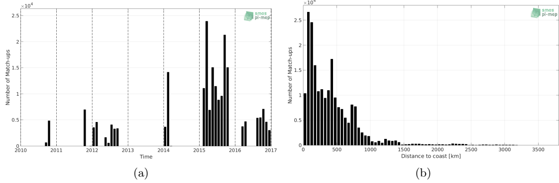
Figure 1: Number of match-ups between TSG-GOSUD-Research-vessel and SMOS-L3-CATDS-CPDC-V3-10DAYS-25KM SSS as a function of time (a) and as function of the distance to coast (b) over the South Pacific Ocean Pi-MEP region and for the full satellite product period.
