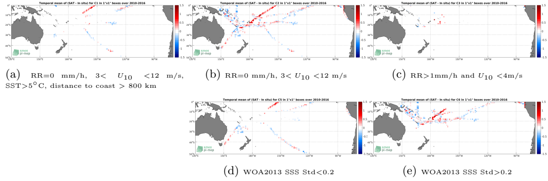
Figure 12: Temporal mean gridded over spatial boxes of size 1^\circ \times 1^\circ of \Delta SSS (SMOS-L3-CATDS-CPDC-V3-10DAYS-25KM - TSG-GOSUD-Research-vessel) for 5 different subdatasets corresponding to: RR=0 mm/h, 3 < U_{10} < 12 m/s, SST > 5^\circ C , distance to coast > 800 km (a), RR=0 mm/h, 3 < U_{10} < 12 m/s (b), RR > 1 mm/h and U_{10} < 4 m/s (c), WOA2013 SSS Std < 0.2 (d), WOA2013 SSS Std > 0.2 (e).
