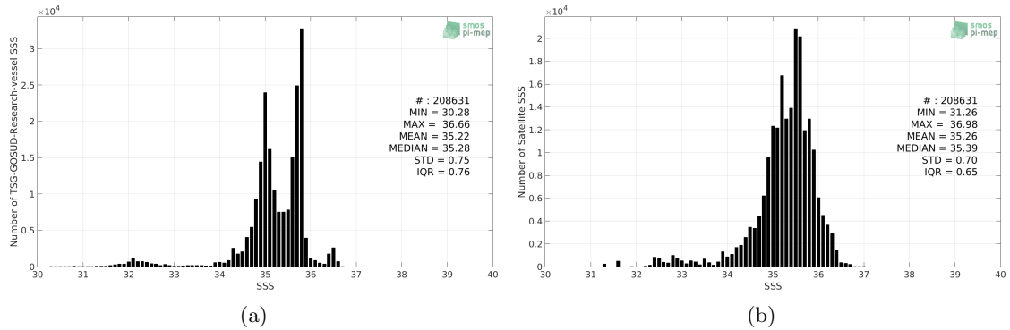
Figure 2: Histograms of SSS from TSG-GOSUD-Research-vessel (a) and SMOS-L3-CATDS-CPDC-V3-10DAYS-25KM (b) considering all match-up pairs per bins of 0.1 over the South Pacific Ocean Pi-MEP region and for the full satellite product period.
