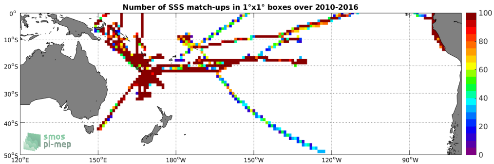
Figure 4: Number of SSS match-ups between TSG-GOSUD-Research-vessel SSS and the SMOS-L3-CATDS-CPDC-V3-10DAYS-25KM SSS product for the South Pacific Ocean Pi-MEP region over 1^\circ \times 1^\circ boxes and for the full satellite product period.
