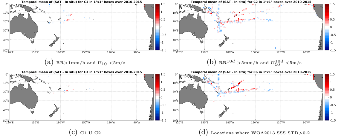
Figure 12: Temporal mean gridded over spatial boxes of size 1^\circ \times 1^\circ of \Delta SSS (SMOS-L3-CATDS-CPDC-V3-10DAYS-25KM - TSG-GOSUD-Research-vessel) for 4 different subdatasets corresponding to: RR > 1mm/h and U_{10} < 5 m/s (a), RR^{10d} > 5 mm/h and U_{10}^{10d} < 5 m/s (b), C1 U C2 (c), Locations where WOA2013 SSS STD > 0.2 (d).
