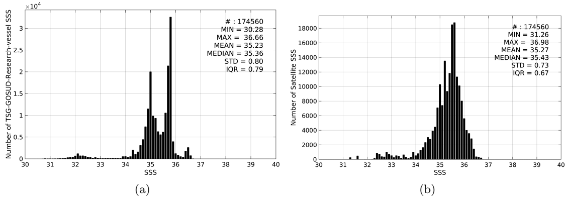
Figure 2: Histograms of SSS from TSG-GOSUD-Research-vessel (a) and SMOS-L3-CATDS-CPDC-V3-10DAYS-25KM (b) considering all match-up pairs per bins of 0.1 over the South Pacific Ocean Pi-MEP region and for the full satellite product period.
