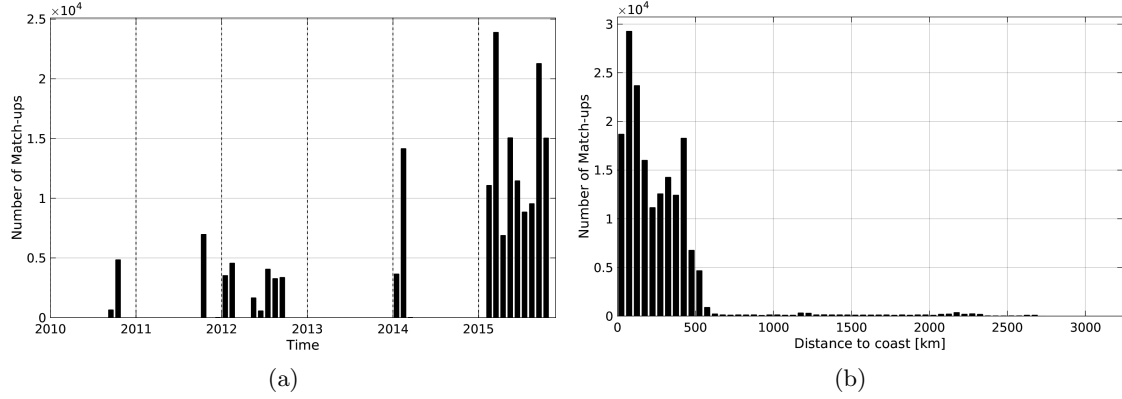
Figure 1: Number of match-ups between TSG-GOSUD-Research-vessel and SMOS-L3-CATDS-CPDC-V3-10DAYS-25KM SSS as a function of time (a) and as function of the distance to coast (b) over the South Pacific Ocean Pi-MEP region and for the full satellite product period.
