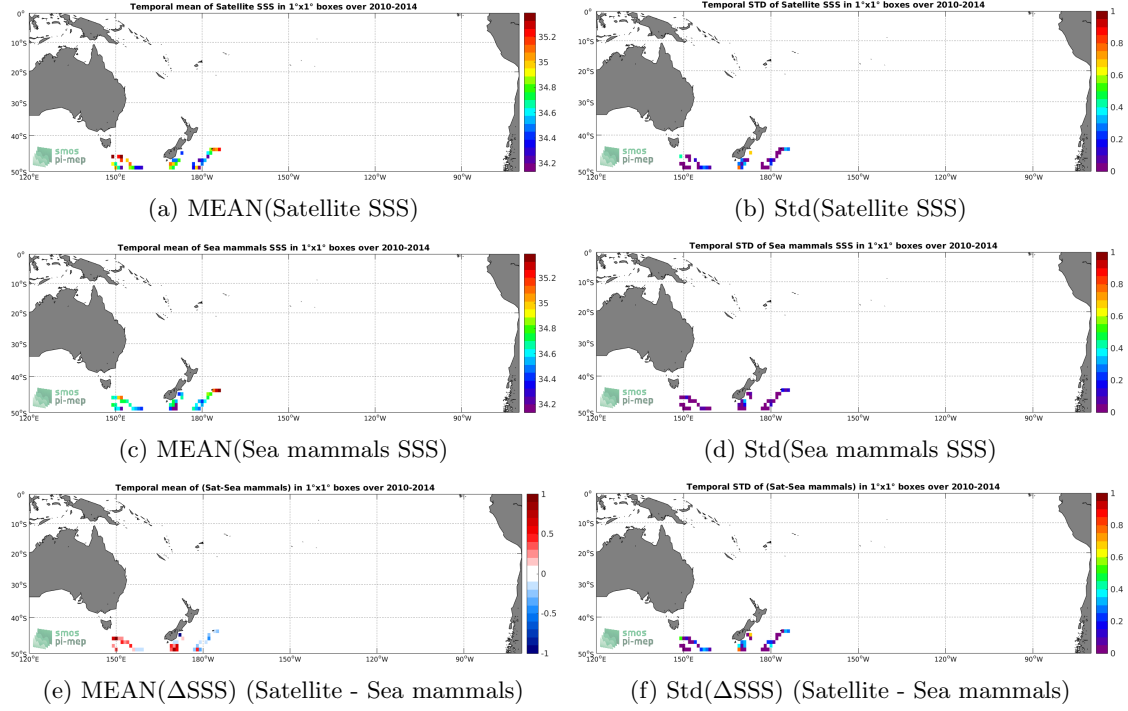
Figure 6: Temporal mean (left) and Std (right) of SSS from SMOS-L3-CATDS-CPDC-V3-10DAYS-25KM (top), Sea mammals (middle), and of \Delta SSS (Satellite - Sea mammals). Only match-up pairs are used to generate these maps.
