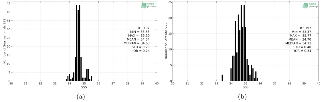
Figure 2: Histograms of SSS from Sea mammals (a) and SMOS-L3-CATDS-CPDC-V3-10DAYS-25KM (b) considering all match-up pairs per bins of 0.1 over the South Pacific Ocean Pi-MEP region and for the full satellite product period.
