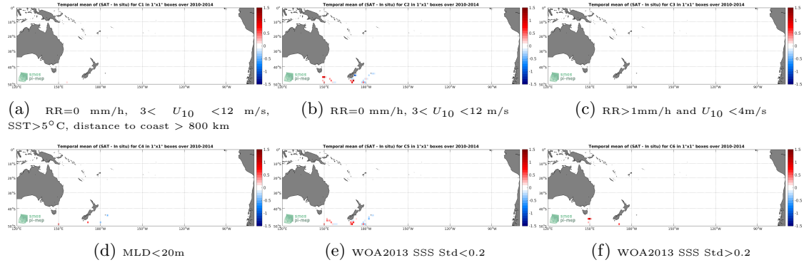
Figure 12: Temporal mean gridded over spatial boxes of size 1^\circ \times 1^\circ of \Delta SSS (SMOS-L3-CATDS-CPDC-V3-10DAYS-25KM - Sea mammals) for 6 different subdatasets corresponding to: RR=0 mm/h, 3 < U_{10} < 12 m/s, SST > 5^\circ C , distance to coast > 800 km (a), RR=0 mm/h, 3 < U_{10} < 12 m/s (b), RR > 1 mm/h and U_{10} < 4 m/s (c), MLD < 20 m (d), WOA2013 SSS Std < 0.2 (e), WOA2013 SSS Std > 0.2 (f).
