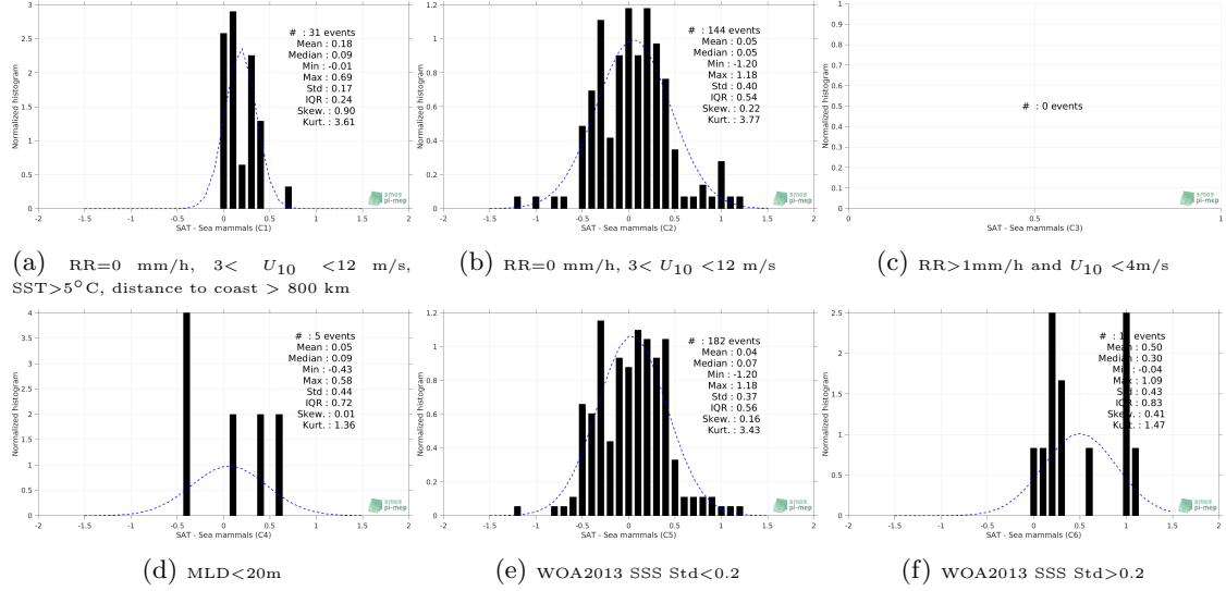
Figure 13: Normalized histogram of \Delta\text{SSS} (SMOS-L3-CATDS-CPDC-V3-10DAYS-25KM - Sea mammals) for 6 different subdatasets corresponding to: RR=0 mm/h, 3 < U_{10} < 12 m/s, SST > 5^{\circ}\text{C} , distance to coast > 800 km (a), RR=0 mm/h, 3 < U_{10} < 12 m/s (b), RR > 1 mm/h and U_{10} < 4 m/s (c), MLD < 20 m (d), WOA2013 SSS Std < 0.2 (e), WOA2013 SSS Std > 0.2 (f).
