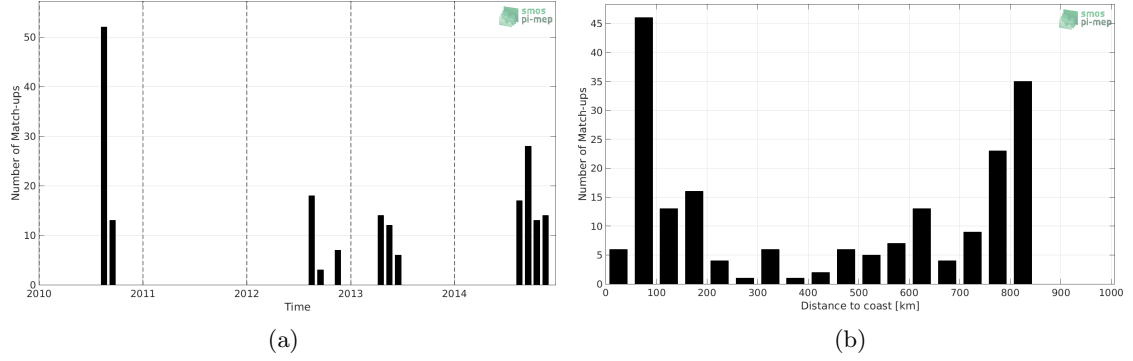
Figure 1: Number of match-ups between Sea mammals and SMOS-L3-CATDS-CPDC-V3-10DAYS-25KM SSS as a function of time (a) and as function of the distance to coast (b) over the South Pacific Ocean Pi-MEP region and for the full satellite product period.
