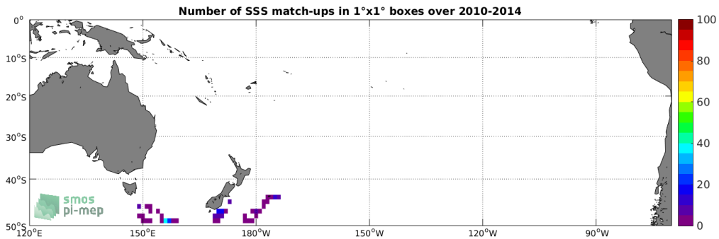
Figure 4: Number of SSS match-ups between Sea mammals SSS and the SMOS-L3-CATDS-CPDC-V3-10DAYS-25KM SSS product for the South Pacific Ocean Pi-MEP region over 1^\circ \times 1^\circ boxes and for the full satellite product period.
