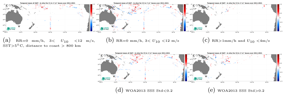
Figure 14: Temporal mean gridded over spatial boxes of size 1^\circ \times 1^\circ of \Delta\text{SSS} (SMOS SSS L3 v2 - 9-Days (BEC) - TSG (SAMOS)) for 5 different subdatasets corresponding to:RR=0 mm/h, 3 < U_{10} < 12 m/s, SST >5^\circ\text{C} , distance to coast > 800 km (a), RR=0 mm/h, 3 < U_{10} < 12 m/s (b), RR >1 mm/h and U_{10} < 4 m/s (c), WOA2013 SSS Std <0.2 (d), WOA2013 SSS Std >0.2 (e).
