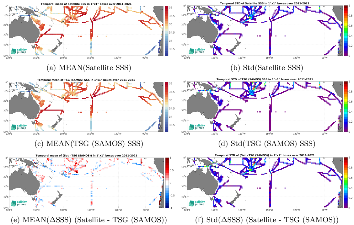
Figure 7: Temporal mean (left) and Std (right) of SSS from SMOS SSS L3 v2 - 9-Days (BEC) (top), TSG (SAMOS) (middle), and of \Delta SSS (Satellite - TSG (SAMOS)). Only match-up pairs are used to generate these maps.
