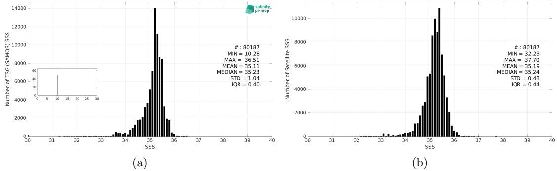
Figure 3: Histograms of SSS from TSG (SAMOS) (a) and SMOS SSS L3 v2 - 9-Days (BEC) (b) considering all match-up pairs per bins of 0.1 over the South Pacific Ocean Pi-MEP region and for the full satellite product period.
