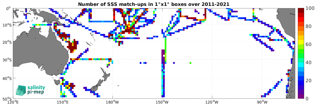
Figure 5: Number of SSS match-ups between TSG (SAMOS) SSS and the SMOS SSS L3 v2 - 9-Days (BEC) SSS product for the South Pacific Ocean Pi-MEP region over 1^\circ \times 1^\circ boxes and for the full satellite product period.
