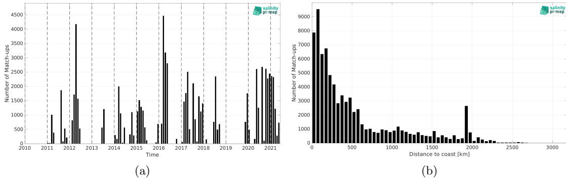
Figure 2: Number of match-ups between TSG (SAMOS) and SMOS SSS L3 v2 - 9-Days (BEC) SSS as a function of time (a) and as function of the distance to coast (b) over the South Pacific Ocean Pi-MEP region and for the full satellite product period.
