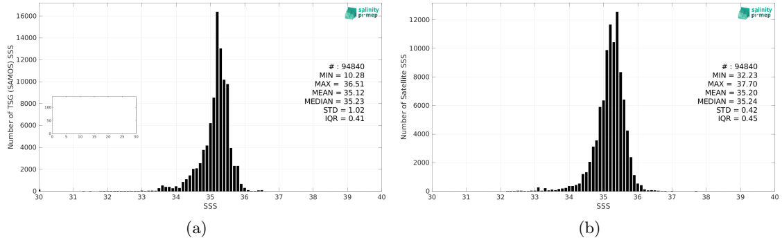
Figure 2: Histograms of SSS from TSG (SAMOS) (a) and SMOS SSS L3 v2 - 9-Days (BEC) (b) considering all match-up pairs per bins of 0.1 over the South Pacific Ocean Pi-MEP region and for the full satellite product period.
