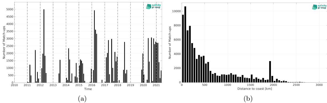
Figure 1: Number of match-ups between TSG (SAMOS) and SMOS SSS L3 v2 - 9-Days (BEC) SSS as a function of time (a) and as function of the distance to coast (b) over the South Pacific Ocean Pi-MEP region and for the full satellite product period.
