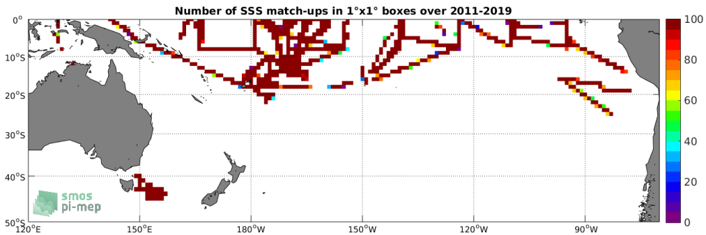
Figure 4: Number of SSS match-ups between TSG (SAMOS) SSS and the SMOS L3 v2 - 9-Days (BEC) SSS product for the South Pacific Ocean Pi-MEP region over 1°x1° boxes and for the full satellite product period.
