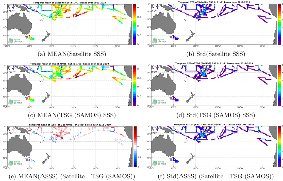
Figure 6: Temporal mean (left) and Std (right) of SSS from SMOS L3 v2 - 9-Days (BEC) (top), TSG (SAMOS) (middle), and of \Delta SSS (Satellite - TSG (SAMOS)). Only match-up pairs are used to generate these maps.
