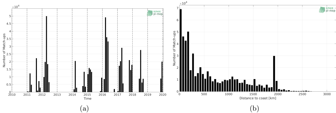
Figure 1: Number of match-ups between TSG (SAMOS) and SMOS L3 v2 - 9-Days (BEC) SSS as a function of time (a) and as function of the distance to coast (b) over the South Pacific Ocean Pi-MEP region and for the full satellite product period.
