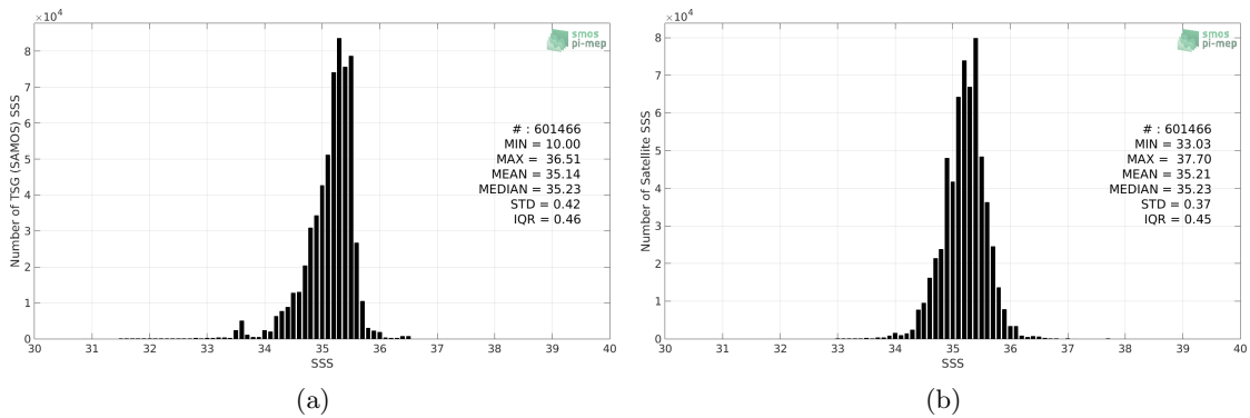
Figure 2: Histograms of SSS from TSG (SAMOS) (a) and SMOS L3 v2 - 9-Days (BEC) (b) considering all match-up pairs per bins of 0.1 over the South Pacific Ocean Pi-MEP region and for the full satellite product period.
