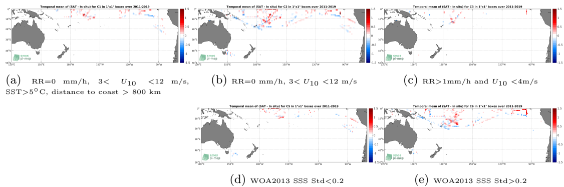
Figure 12: Temporal mean gridded over spatial boxes of size 1^\circ \times 1^\circ of \Delta SSS (SMOS L3 v2 - 9-Days (BEC) - TSG (SAMOS)) for 5 different subdatasets corresponding to:RR=0 mm/h, 3 < U_{10} < 12 m/s, SST >5^\circ\text{C} , distance to coast > 800 km (a), RR=0 mm/h, 3 < U_{10} < 12 m/s (b), RR >1 mm/h and U_{10} < 4 m/s (c), WOA2013 SSS Std <0.2 (d), WOA2013 SSS Std >0.2 (e).
