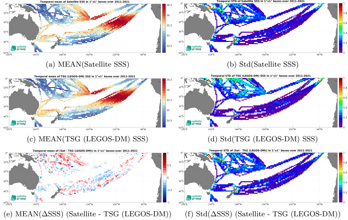
Figure 6: Temporal mean (left) and Std (right) of SSS from SMOS SSS L3 v2 - 9-Days (BEC) (top), TSG (LEGOS-DM) (middle), and of \Delta\text{SSS} (Satellite - TSG (LEGOS-DM)). Only match-up pairs are used to generate these maps.
