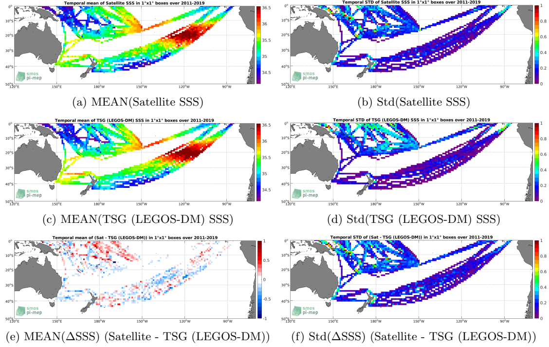
Figure 6: Temporal mean (left) and Std (right) of SSS from SMOS SSS L3 v2 - 9-Days (BEC) (top), TSG (LEGOS-DM) (middle), and of \Delta SSS (Satellite - TSG (LEGOS-DM)). Only match-up pairs are used to generate these maps.
