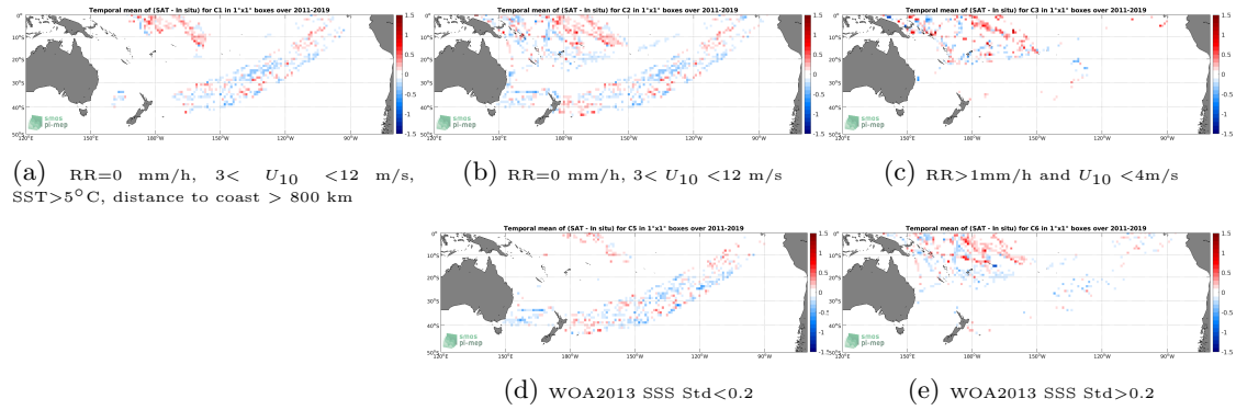
Figure 12: Temporal mean gridded over spatial boxes of size 1^\circ \times 1^\circ of \Delta SSS (SMOS SSS L3 v2 - 9-Days (BEC) - TSG (LEGOS-DM)) for 5 different subdatasets corresponding to: RR=0 mm/h, 3 < U_{10} < 12 m/s, SST > 5^\circ C , distance to coast > 800 km (a), RR=0 mm/h, 3 < U_{10} < 12 m/s (b), RR > 1 mm/h and U_{10} < 4 m/s (c), WOA2013 SSS Std < 0.2 (d), WOA2013 SSS Std > 0.2 (e).
