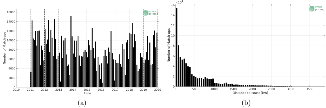
Figure 1: Number of match-ups between TSG (LEGOS-DM) and SMOS SSS L3 v2 - 9-Days (BEC) SSS as a function of time (a) and as function of the distance to coast (b) over the South Pacific Ocean Pi-MEP region and for the full satellite product period.
