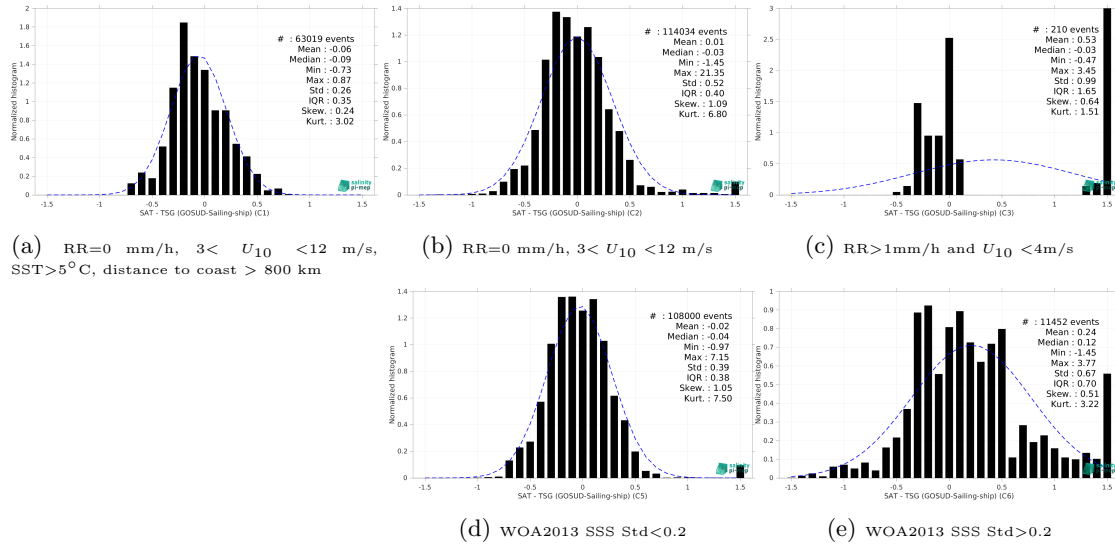
Figure 15: Normalized histogram of \Delta\text{SSS} (SMOS SSS L3 v2 - 9-Days (BEC) - TSG (GOSUD-Sailing-ship)) for 5 different subdatasets corresponding to: RR=0 mm/h, 3 < U_{10} < 12 m/s, SST>5°C, distance to coast > 800 km (a), RR=0 mm/h, 3 < U_{10} < 12 m/s (b), RR>1mm/h and U_{10} < 4 m/s (c), WOA2013 SSS Std<0.2 (d), WOA2013 SSS Std>0.2 (e).
