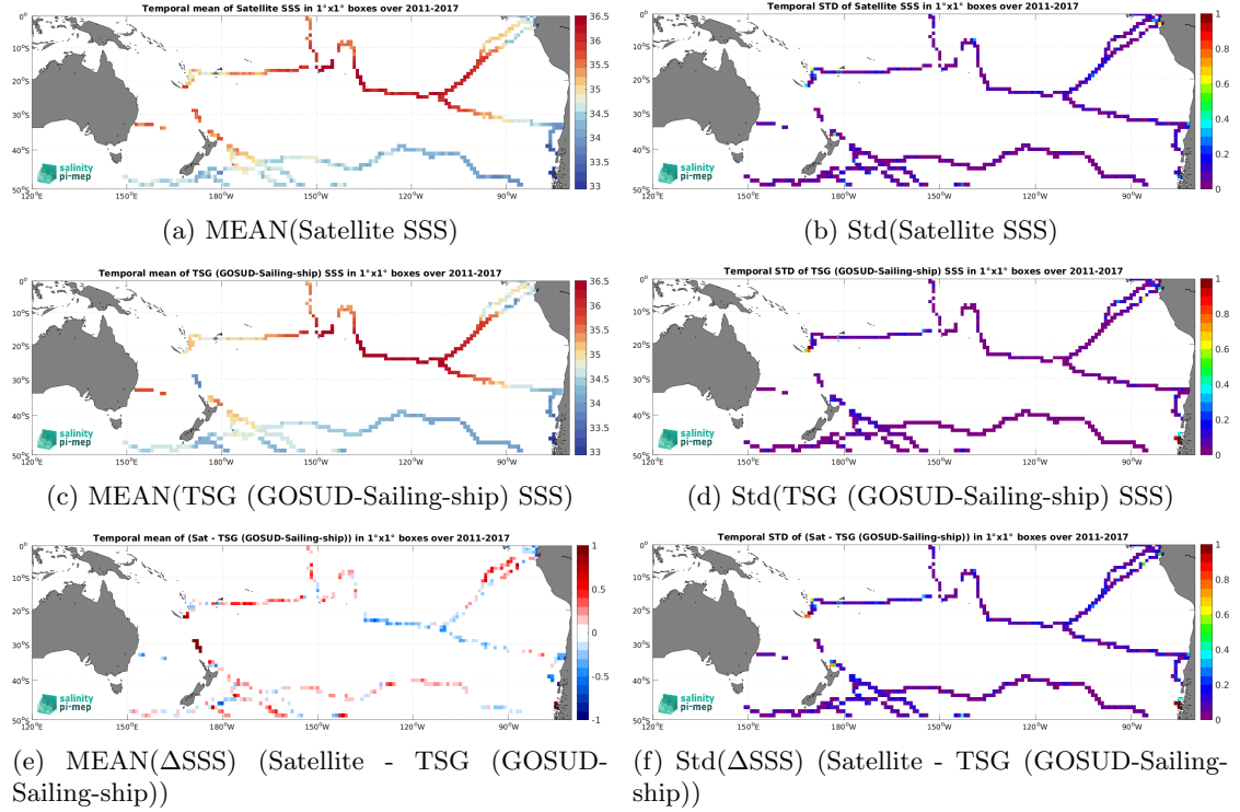
Figure 7: Temporal mean (left) and Std (right) of SSS from SMOS SSS L3 v2 - 9-Days (BEC) (top), TSG (GOSUD-Sailing-ship) (middle), and of \Delta SSS (Satellite - TSG (GOSUD-Sailing-ship)). Only match-up pairs are used to generate these maps.
