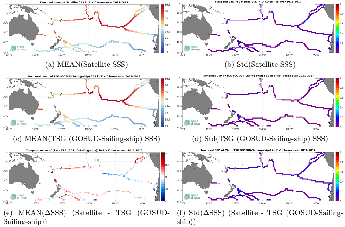
Figure 6: Temporal mean (left) and Std (right) of SSS from SMOS SSS L3 v2 - 9-Days (BEC) (top), TSG (GOSUD-Sailing-ship) (middle), and of \Delta SSS (Satellite - TSG (GOSUD-Sailing-ship)). Only match-up pairs are used to generate these maps.
