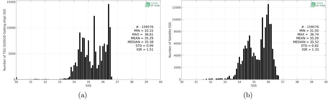
Figure 2: Histograms of SSS from TSG (GOSUD-Sailing-ship) (a) and SMOS SSS L3 v2 - 9-Days (BEC) (b) considering all match-up pairs per bins of 0.1 over the South Pacific Ocean Pi-MEP region and for the full satellite product period.
