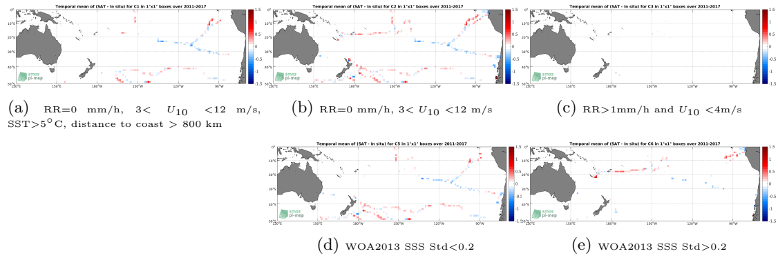
Figure 12: Temporal mean gridded over spatial boxes of size 1^\circ \times 1^\circ of \Delta SSS (SMOS L3 v2 - 9-Days (BEC) - TSG (GOSUD-Sailing-ship)) for 5 different subdatasets corresponding to: RR=0 mm/h, 3 < U_{10} < 12 m/s, SST>5°C, distance to coast > 800 km (a), RR=0 mm/h, 3 < U_{10} < 12 m/s (b), RR>1mm/h and U_{10} < 4 m/s (c), WOA2013 SSS Std<0.2 (d), WOA2013 SSS Std>0.2 (e).
