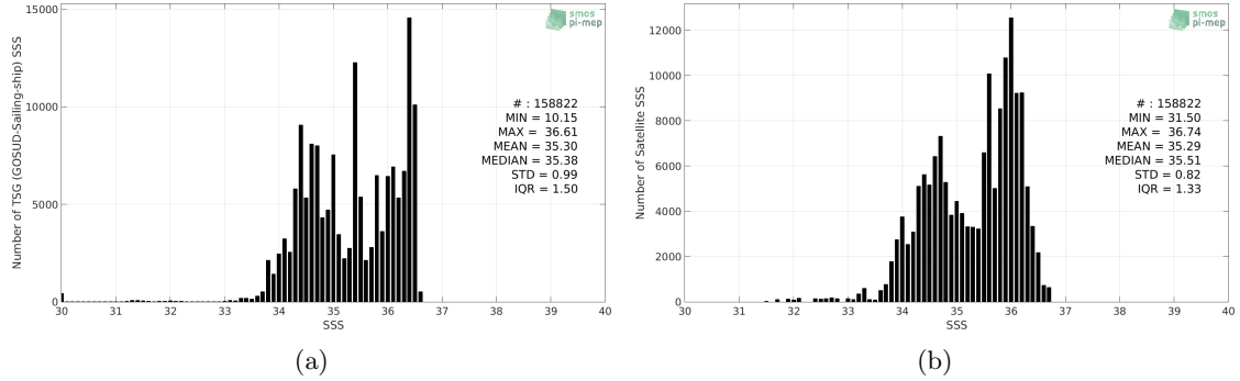
Figure 2: Histograms of SSS from TSG (GOSUD-Sailing-ship) (a) and SMOS L3 v2 - 9-Days (BEC) (b) considering all match-up pairs per bins of 0.1 over the South Pacific Ocean Pi-MEP region and for the full satellite product period.
