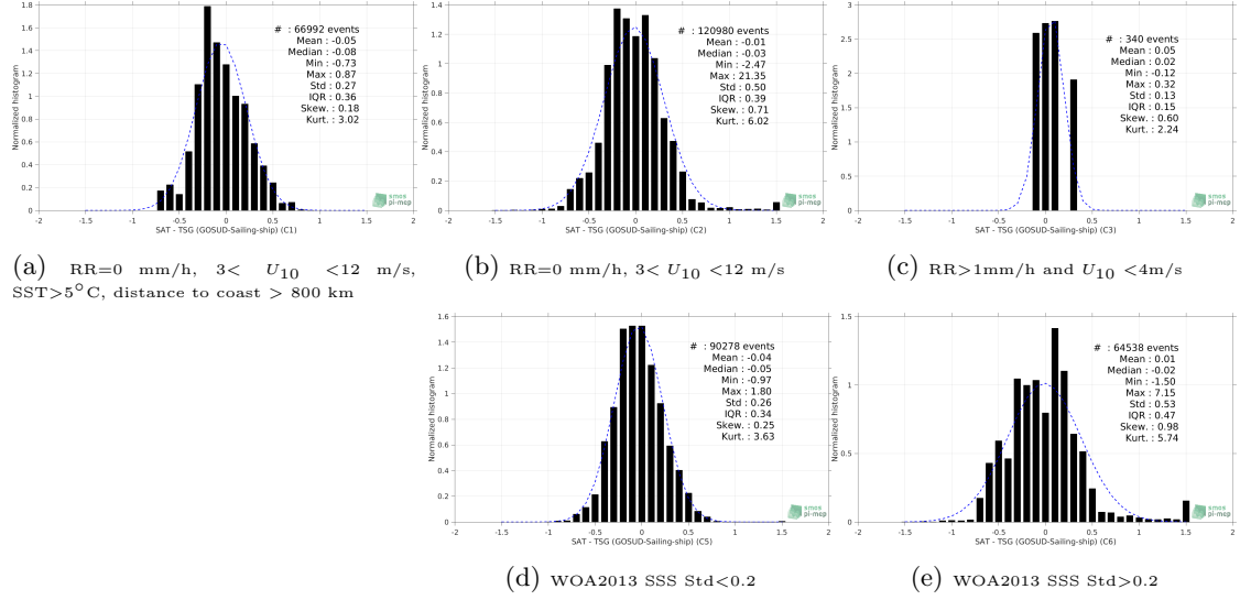
Figure 13: Normalized histogram of \Delta\text{SSS} (SMOS L3 v2 - 9-Days (BEC) - TSG (GOSUD-Sailing-ship)) for 5 different subdatasets corresponding to: RR=0 mm/h, 3 < U_{10} < 12 m/s, SST > 5^\circ\text{C} , distance to coast > 800 km (a), RR=0 mm/h, 3 < U_{10} < 12 m/s (b), RR > 1\text{mm/h} and U_{10} < 4\text{m/s} (c), WOA2013 SSS Std < 0.2 (d), WOA2013 SSS Std > 0.2 (e).
