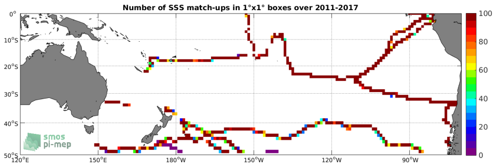
Figure 4: Number of SSS match-ups between TSG (GOSUD-Sailing-ship) SSS and the SMOS L3 v2 - 9-Days (BEC) SSS product for the South Pacific Ocean Pi-MEP region over 1^\circ \times 1^\circ boxes and for the full satellite product period.
