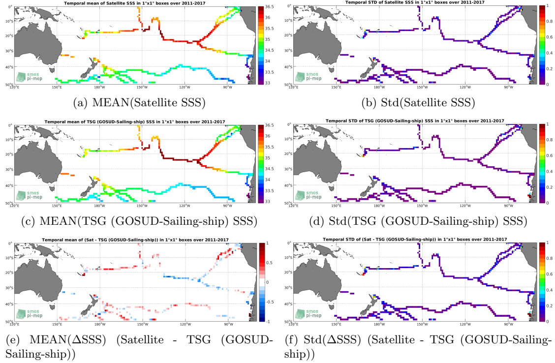
Figure 6: Temporal mean (left) and Std (right) of SSS from SMOS L3 v2 - 9-Days (BEC) (top), TSG (GOSUD-Sailing-ship) (middle), and of \Delta SSS (Satellite - TSG (GOSUD-Sailing-ship)). Only match-up pairs are used to generate these maps.
