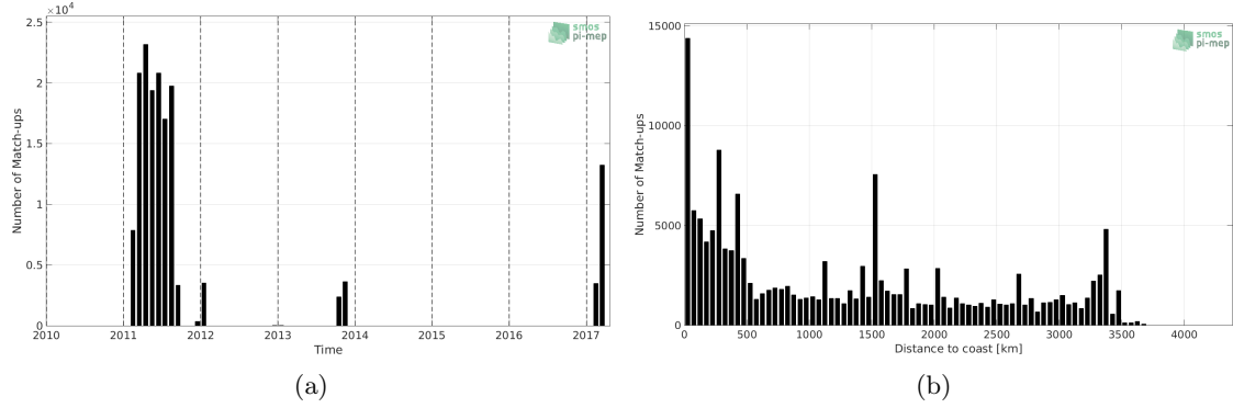
Figure 1: Number of match-ups between TSG (GOSUD-Sailing-ship) and SMOS L3 v2 - 9-Days (BEC) SSS as a function of time (a) and as function of the distance to coast (b) over the South Pacific Ocean Pi-MEP region and for the full satellite product period.
