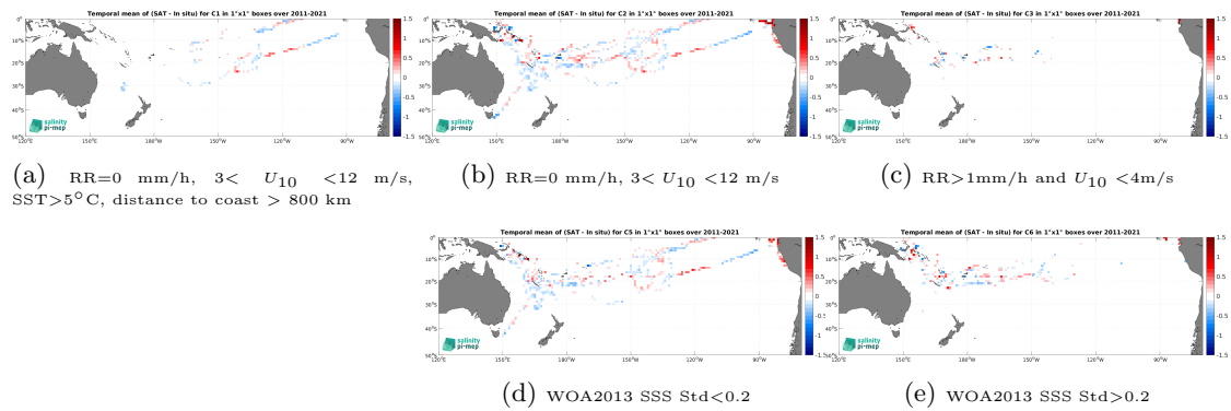
Figure 14: Temporal mean gridded over spatial boxes of size 1^\circ \times 1^\circ of \Delta\text{SSS} (SMOS SSS L3 v2 - 9-Days (BEC) - TSG (GOSUD-Research-vessel)) for 5 different subdatasets corresponding to:RR=0 mm/h, 3 < U_{10} < 12 m/s, SST>5°C, distance to coast > 800 km (a), RR=0 mm/h, 3 < U_{10} < 12 m/s (b), RR>1mm/h and U_{10} < 4 m/s (c), WOA2013 SSS Std<0.2 (d), WOA2013 SSS Std>0.2 (e).
